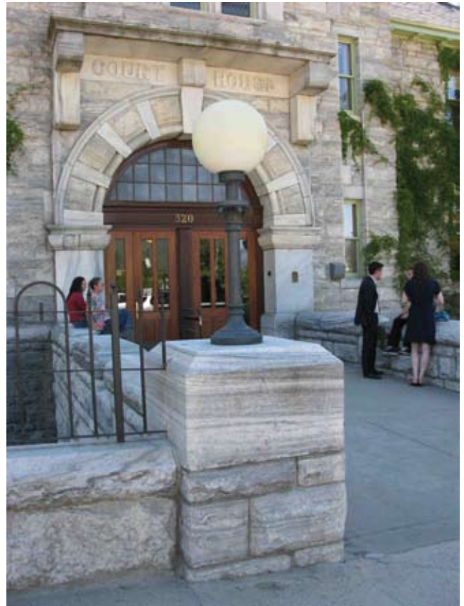
Figure 13. (Right) The Nelson Courthouse is built of marble blocks cut from a quarry north of Kaslo. White layers contain coarse grains of calcite up to 1 cm in diameter, while grey bands are finer grained. Marble is made of intergrown calcite grains that are strong yet easily cut by steel tools, and so are favoured as a building stone.
