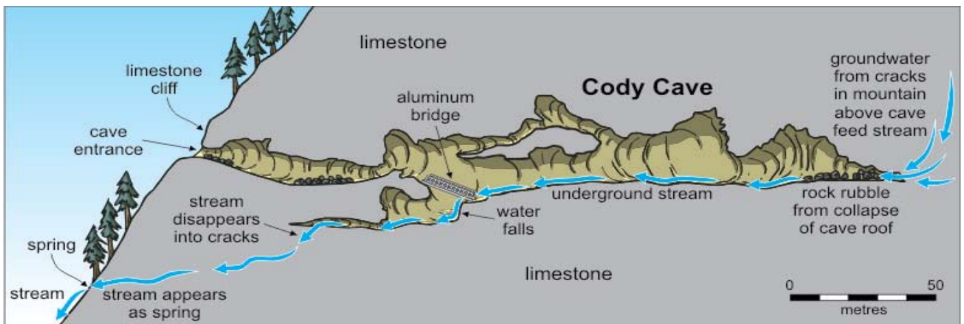
Figure 42. (Below) A cross-section map of Cody Caves. Approximately 800 m of cave is accessible to explorers. An underground stream flows along the floor of the cave.
