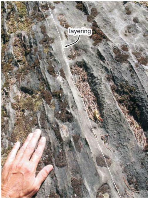
Figure 18. (Above) Rock exposed along the trail to the lookout in Gyro Park is a dark green layered volcanic rock. The rock contains thin layers of different compositions that weather at different rates. More resistant layers form ribs on the rock surface. This is a volcanic rock, altered to green minerals by elevated temperatures and pressures during burial deep in the earth. (Left) Close up of volcanic rock. The layers may represent volcanic ash beds deposited near an ancient volcano.
