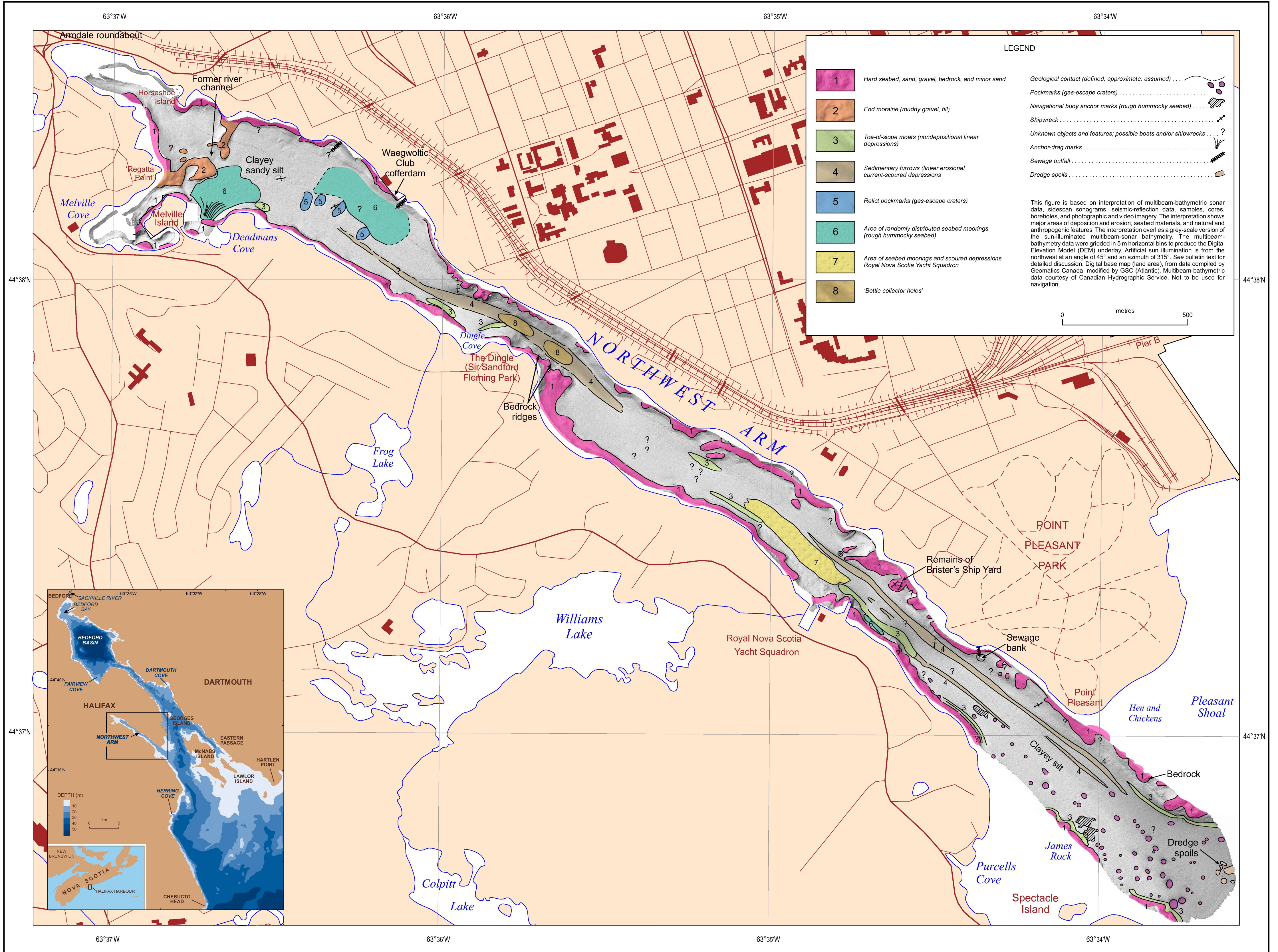
Figure 103. Interpretation of seabed morphology, features, and processes of the Northwest Arm, Halifax Harbour, Nova Scotia; inset is the location map with bathymetry.
