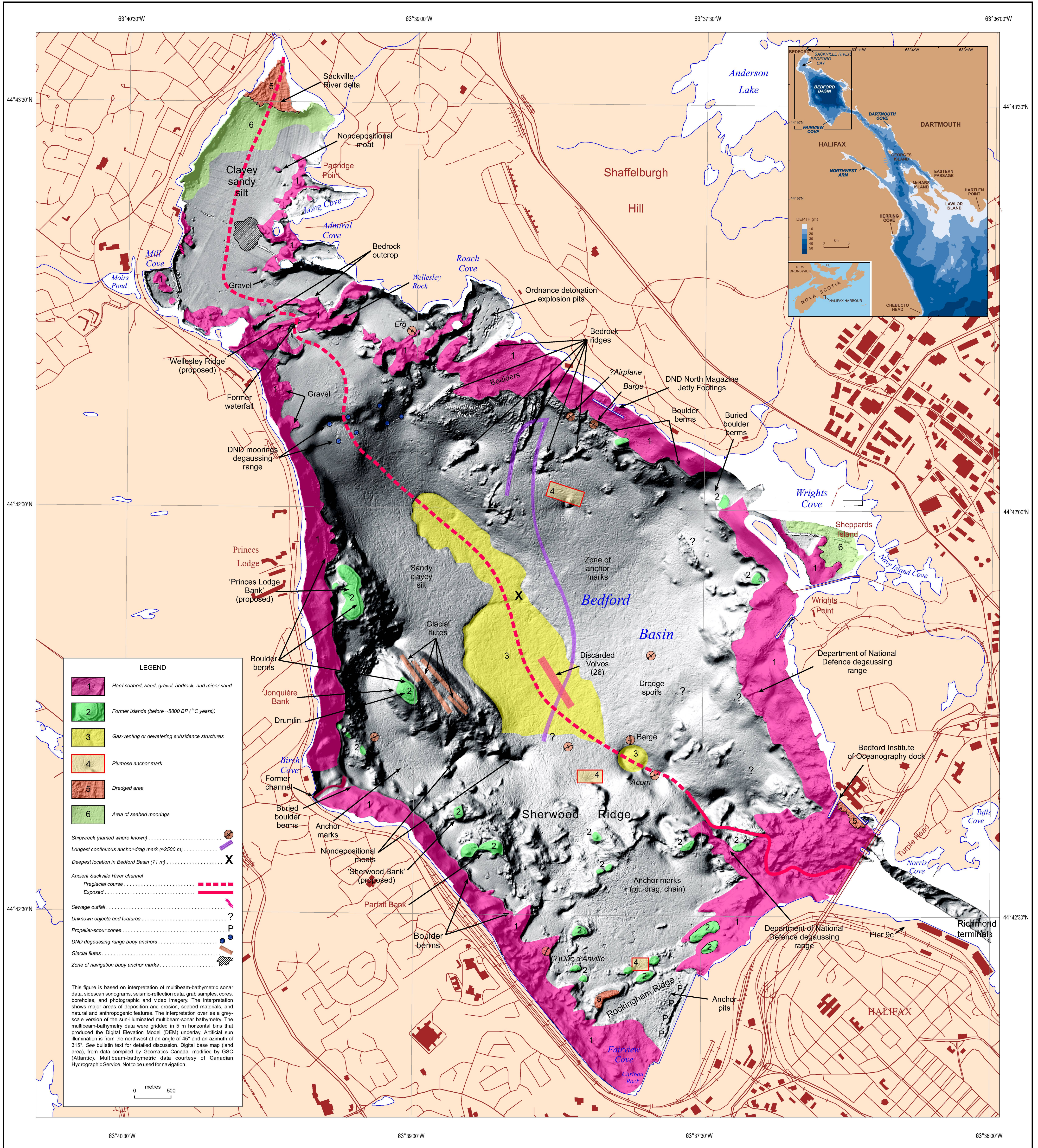
Figure 18. Interpretation of seabed morphology, features, and processes of Bedford Basin, Halifax Harbour, Nova Scotia; inset is the location map with bathymetry.
