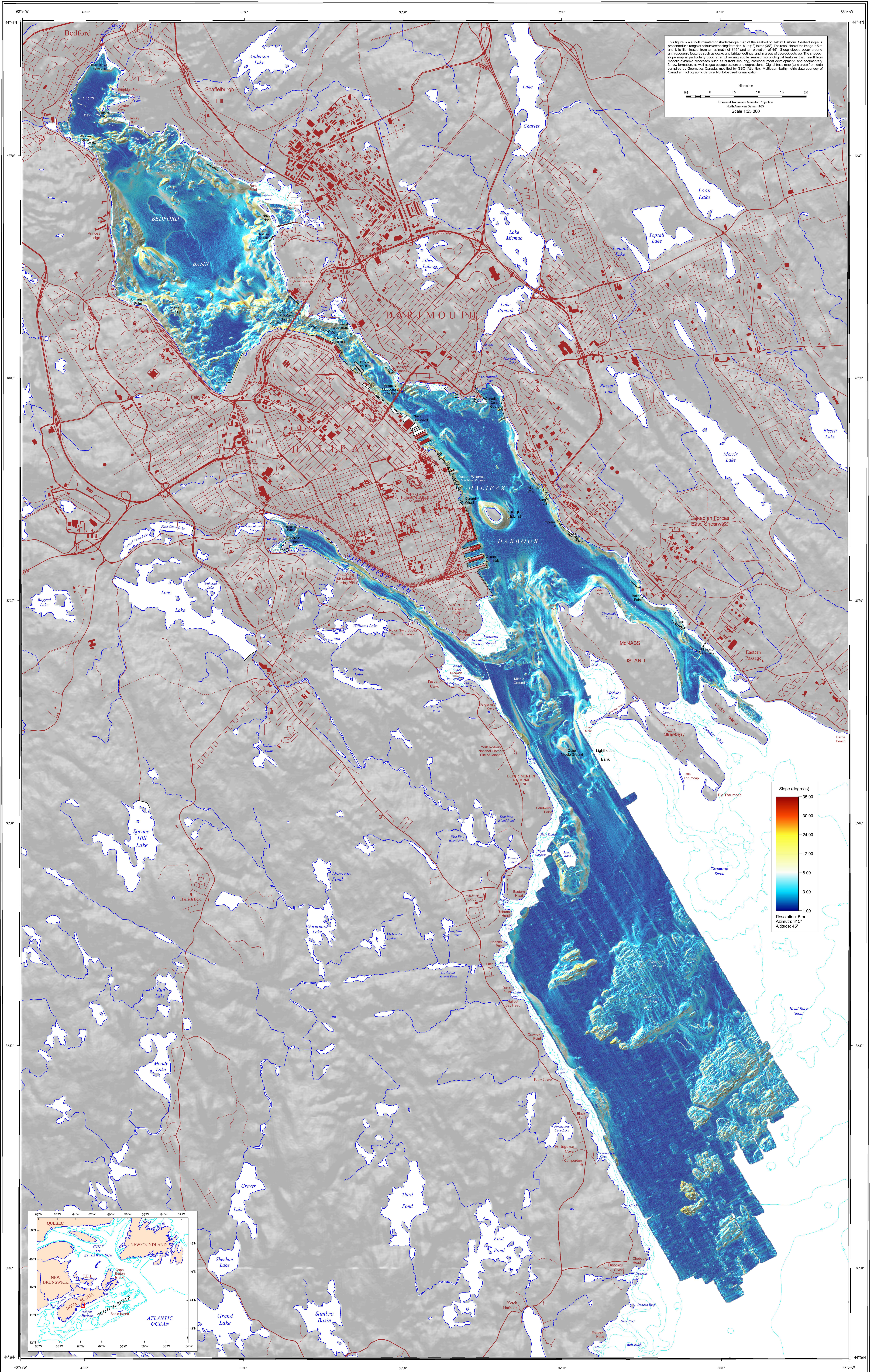
Figure 12. Sun-illuminated seabed slope, Bedford Bay to Chebucto Head, Halifax Harbour, Nova Scotia; inset is the location map.
