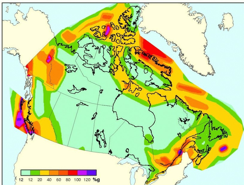
Figure 2. S_a(0.2) for Canada (median values of 5% damped spectral acceleration for Site Class C and a probability of 2%/50 years).
