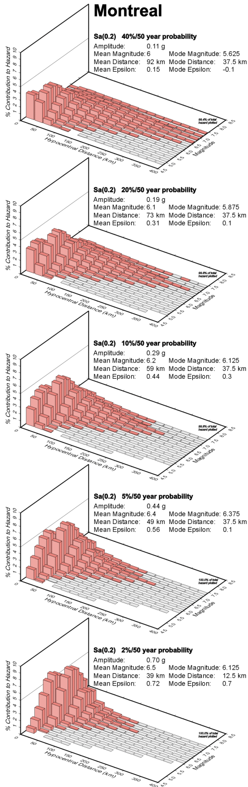
Figure 4. Deaggregation of Montreal and Vancouver Sa(0.2) for increasingly lower probabilities. For Vancouver, the location of the deterministic Cascadia source (not deaggregated) is shown by the blue oval.
