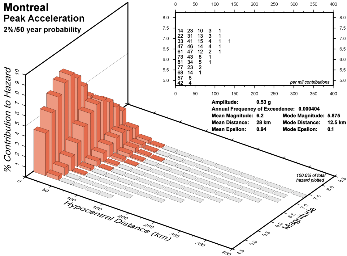
Figure 3. Deaggregation of Montreal PGA for a probability of 2%/50 years. Numerical values in the upper right box allow for an analytical examination ( per mil contributions, divide by 10 to obtain percent contributions). Red bins indicate contributions of at least 1/10 of a percent.
