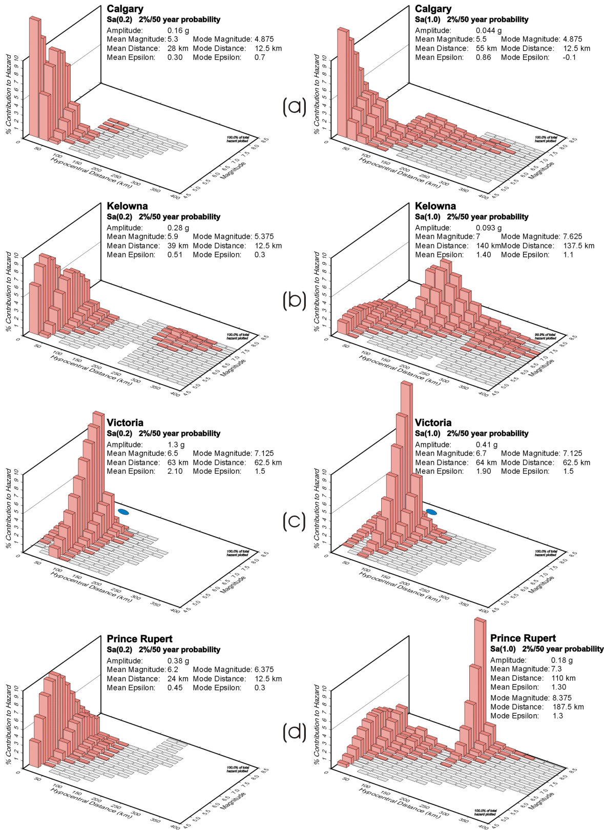
Figure 7. Deaggregation of selected western cities Sa(0.2) and Sa(1.0) hazard for a probability of 2%/50 years.
