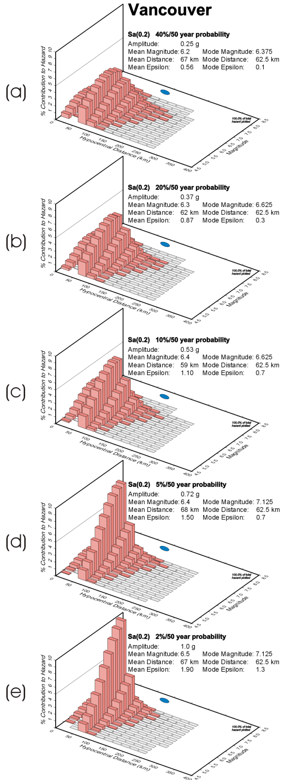
Figure 4. Deaggregation of Montreal and Vancouver Sa(0.2) for increasingly lower probabilities. For Vancouver, the location of the deterministic Cascadia source (not deaggregated) is shown by the blue oval.
