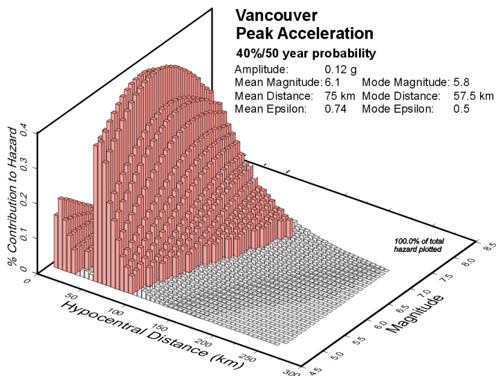
Figure 2. Deaggregation of Vancouver PGA using small-sized bins (5 km distance and 0.1 magnitude units). Although the smoothly varying surface better reflects the magnitude distance distribution, interpretation of the results is difficult as each bin contributes a very small increment of hazard (note vertical scale is in tenths of a percent).
