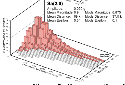
Figure 5. Deaggregation of Montreal and Vancouver for a probability of 2%/50 years for increasingly longer spectral periods.
