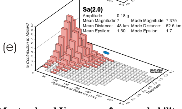
Figure 5. Deaggregation of Montreal and Vancouver for a probability of 2%/50 years for increasingly longer spectral periods.
