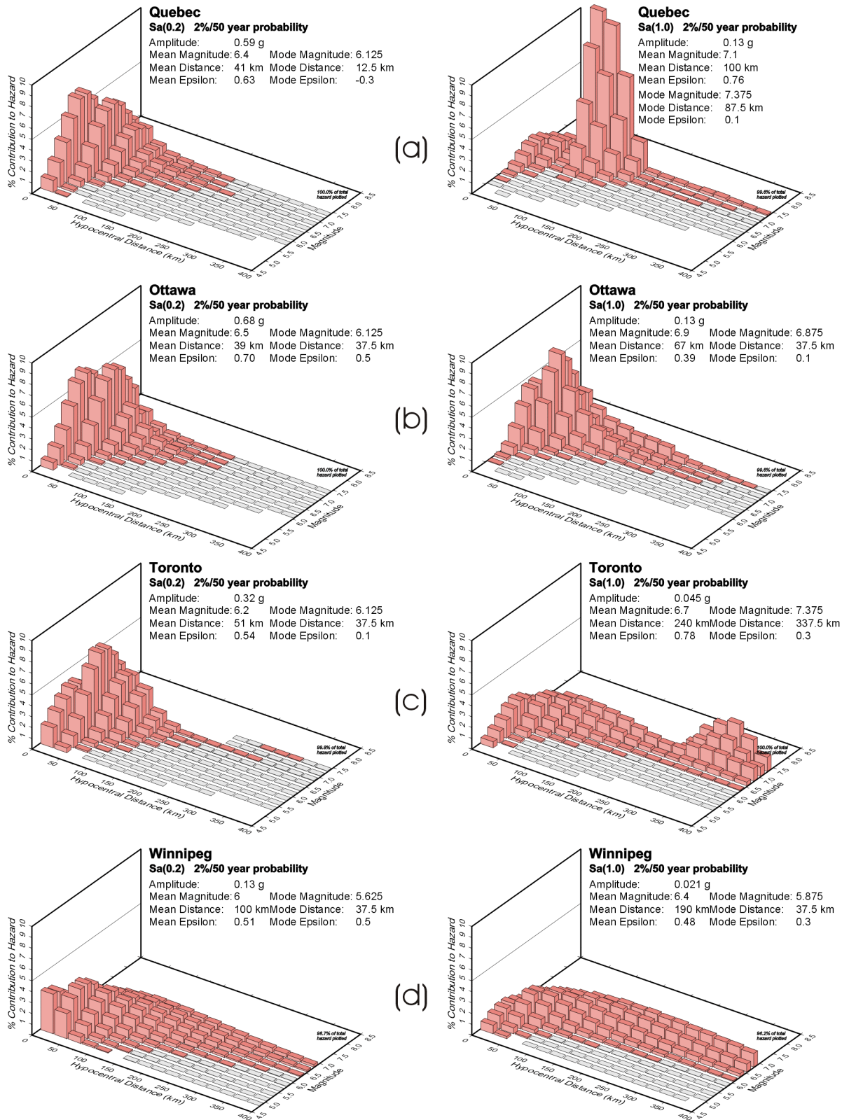
Figure 6. Deaggregation of selected eastern cities Sa(0.2) and Sa(1.0) hazard for a probability of 2%/50 years.
