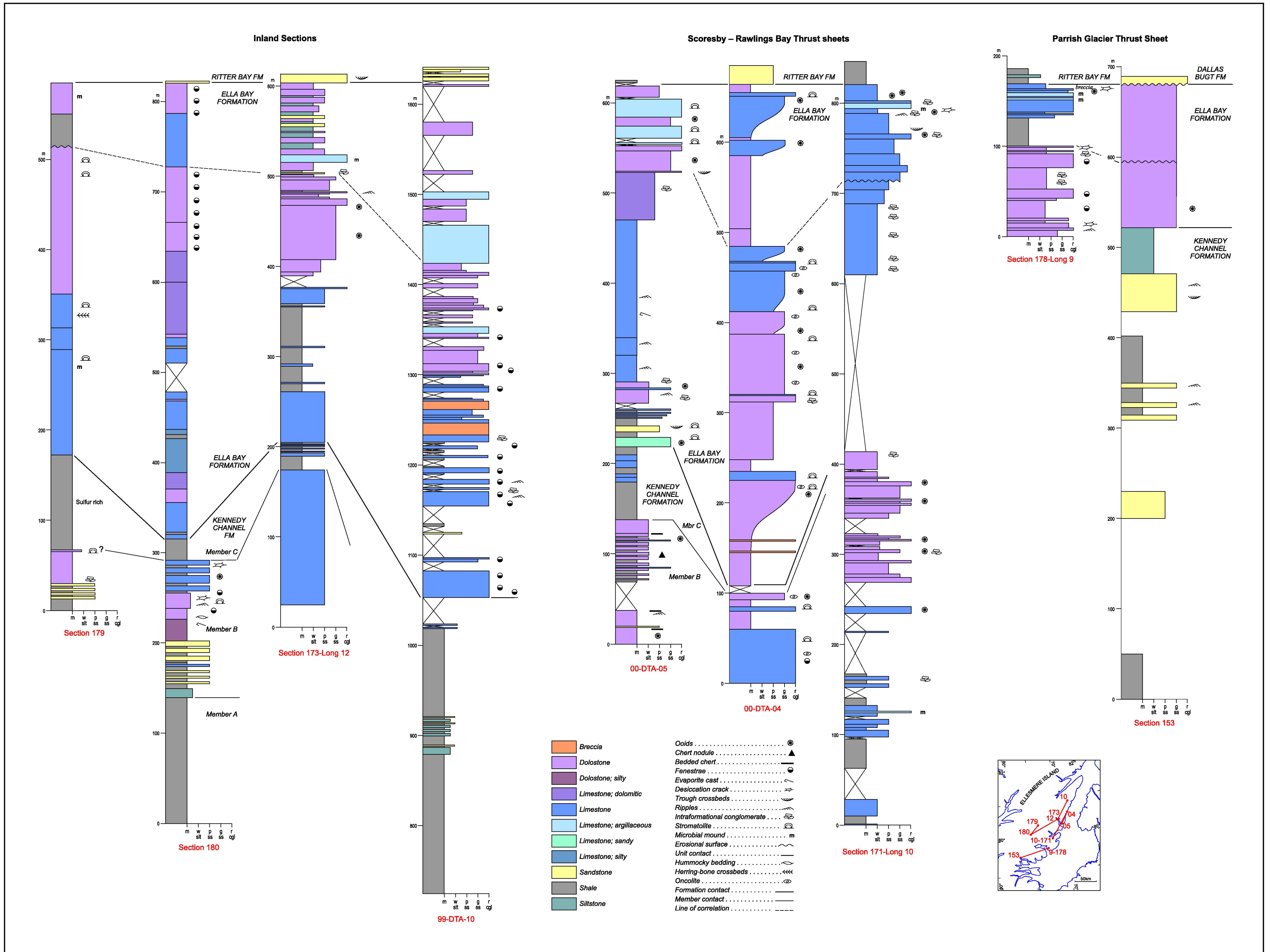
Figure 5. Columnar stratigraphic sections, Kennedy Channel and Ella Bay formations
