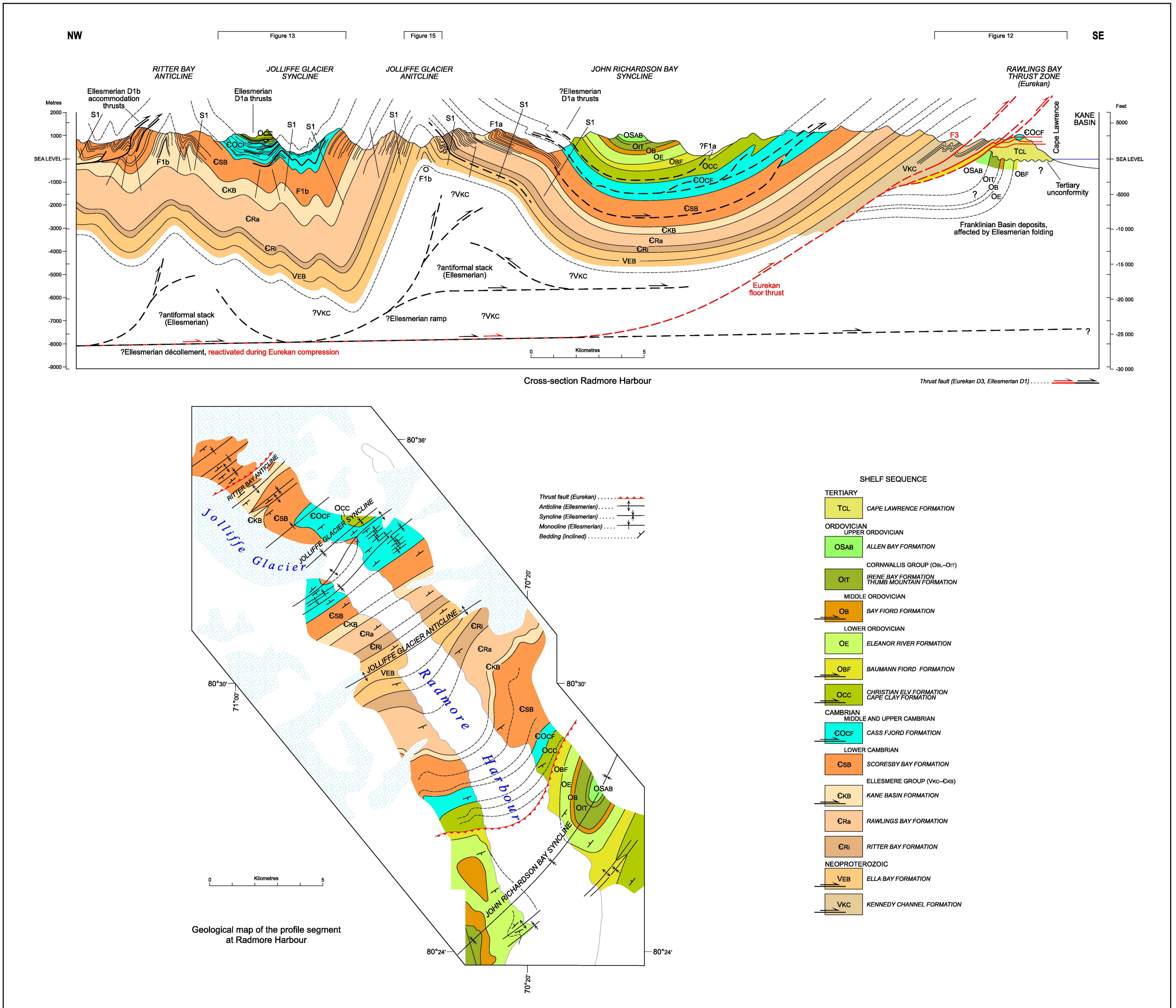
Figure 9. Radmore Harbour cross-section and schematic subsurface interpretation through the Central Ellesmere Fold Belt between Jolliffe Glacier in the northwest and Cape Lawrence in the southeast (for location, see Fig. 1)
