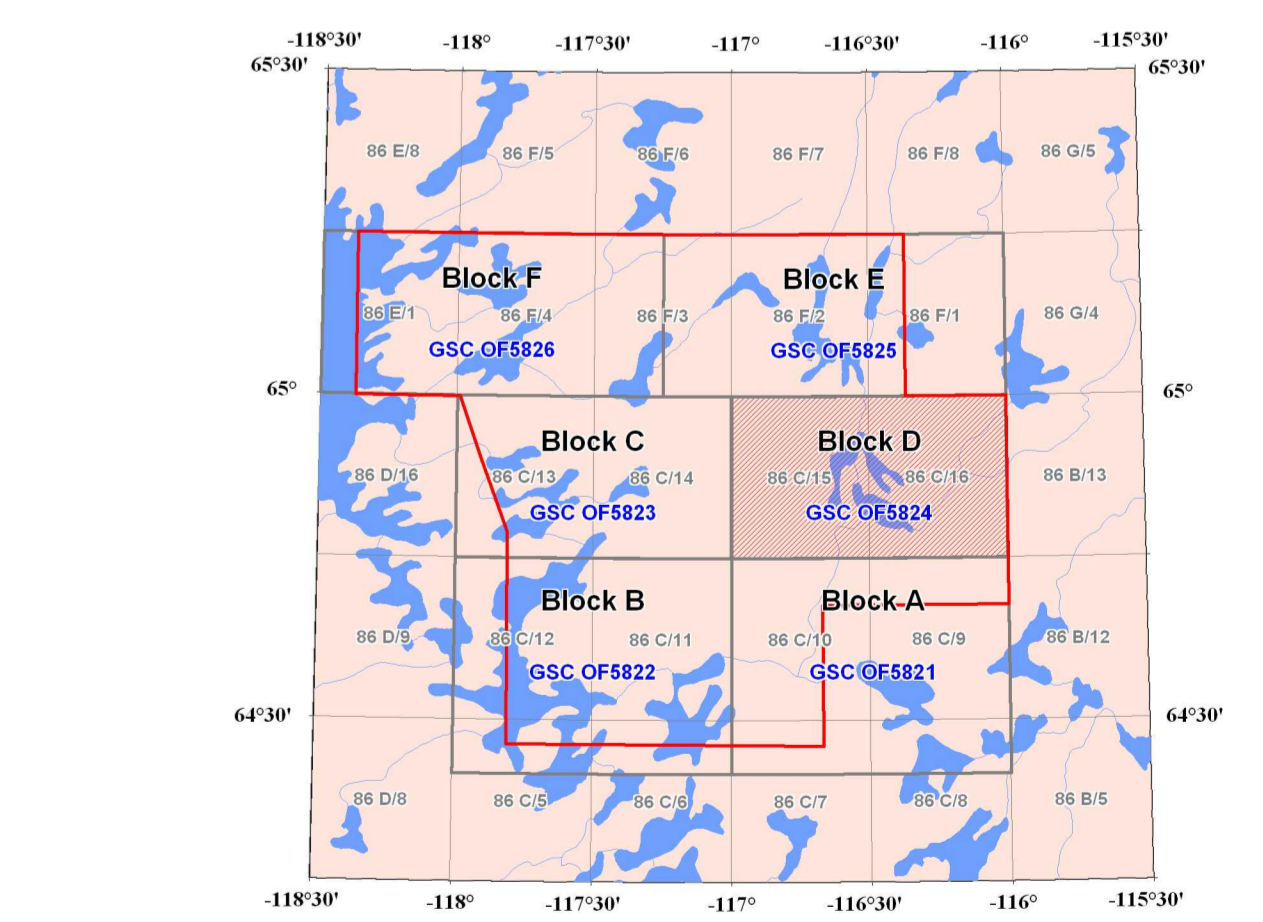
Southwestern Wopmay Orogen parts of 86 C, 86 E, and 86 F
