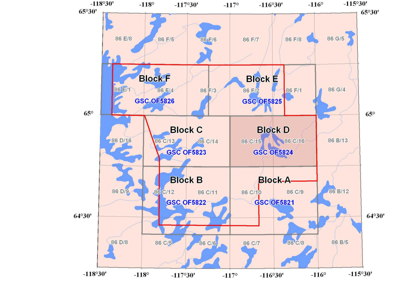
Southwestern Wopmay Orogen parts of 86 C, 86 E, and 86 F
