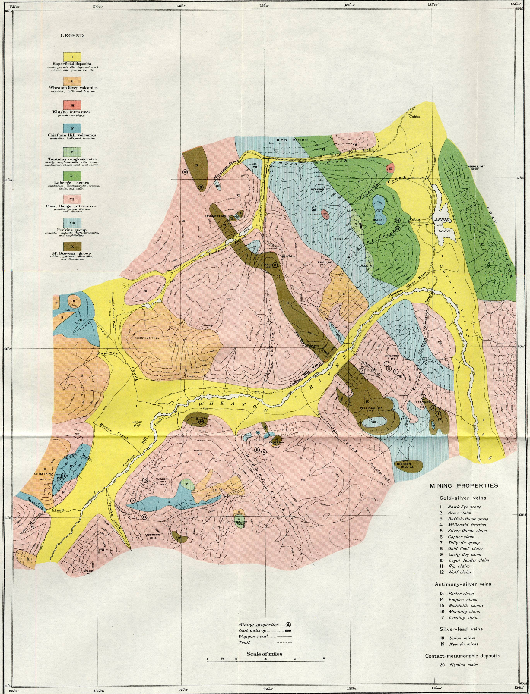
DIAGRAM OF WHEATON MAP-AREA, YUKON; GEOLOGY BY D. D. CAIRNES, 1909.
