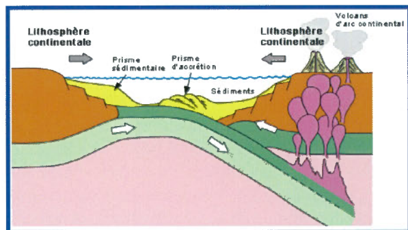
Formation of the Appalachians around the Quebec City region. This episode is represented by the advent of the Quebec City thrust sheet, creating the promontory on which we now stand. http://www.ggl.ulaval.ca/personnel/bourque/intro.pt/planete_terre.html
