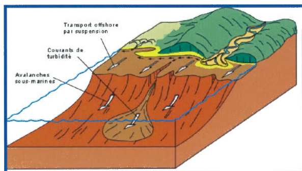
Morphology of the passive continental margin, during the formation of the St. Lawrence Platform. Adapted from: http://www.ggl.ulaval.ca/personnel/bourque/intro.pt/planete_terre.html
