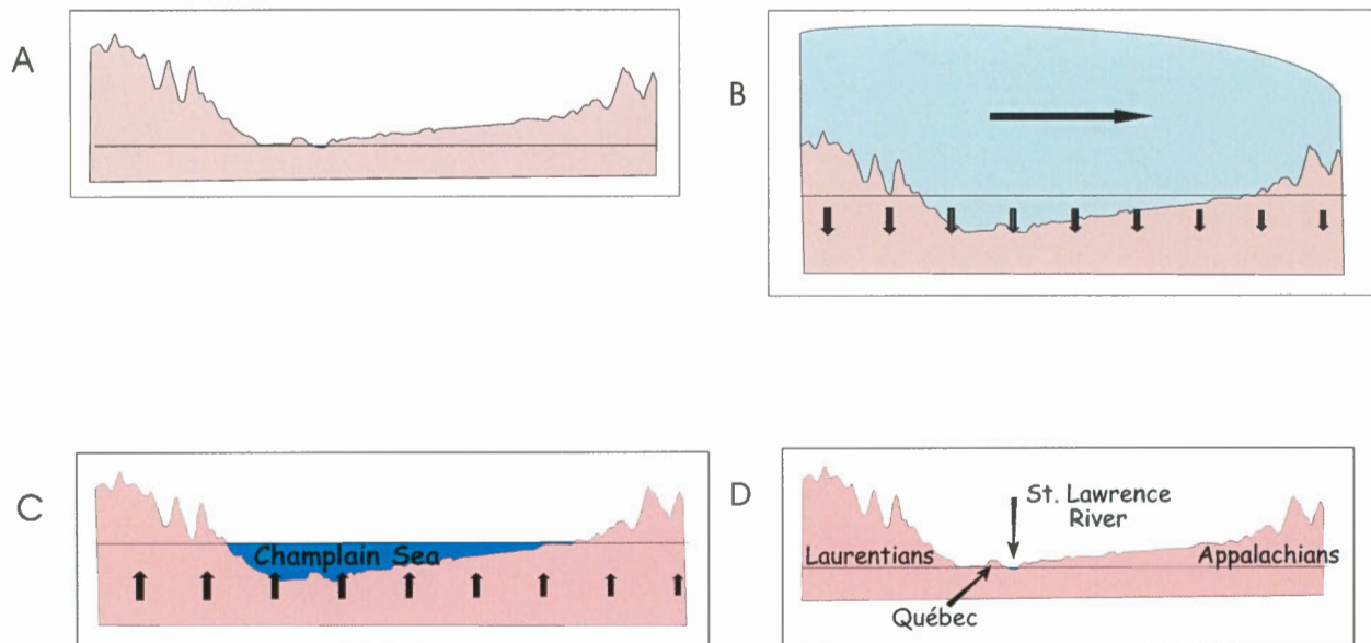
The Champlain Sea occupied the St. Lawrence Valley, sea level declined gradually, isostatic rebound occurred.
