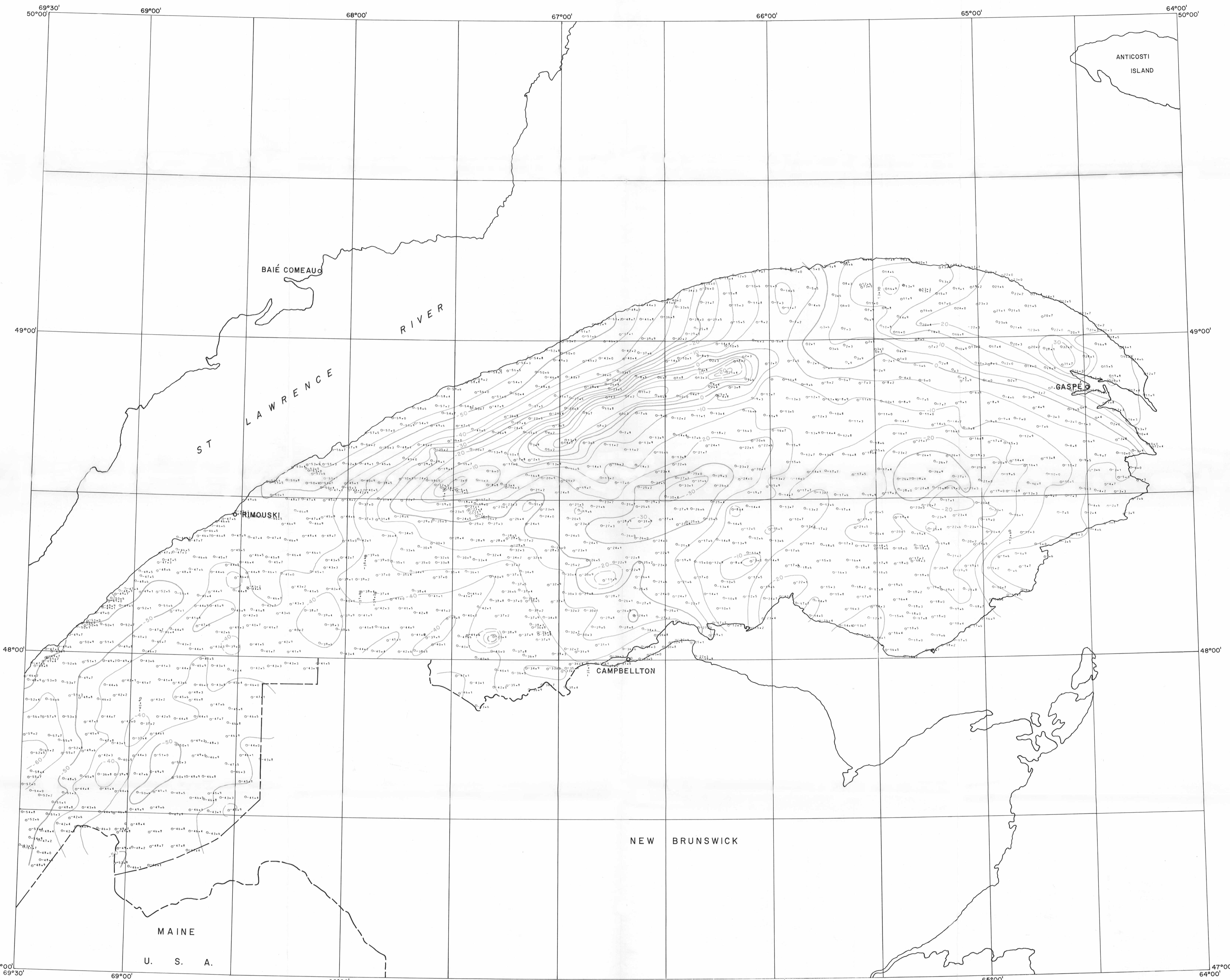
—BOUGUER ANOMALY MAP— Scale 1:500,000 Projection U.T.M.
