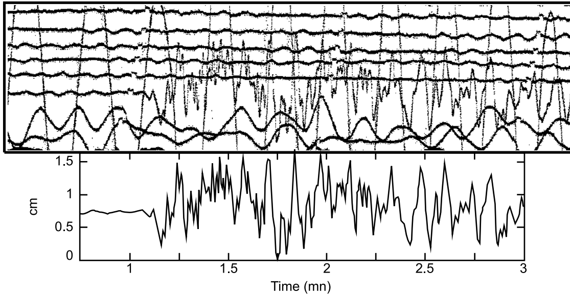
FIGURE 4: Top: Close-up of the P-wave arrival of the 1939 Chilean intraslab earthquake, as recorded on the Pasadena-Benioff 1-100 north-south instrument (tick marks are minutes). Bottom: After optical magnification, such records can be successfully digitized at a rate of 10 samples per second and processed through Newman and Okal's [1998] algorithm.
