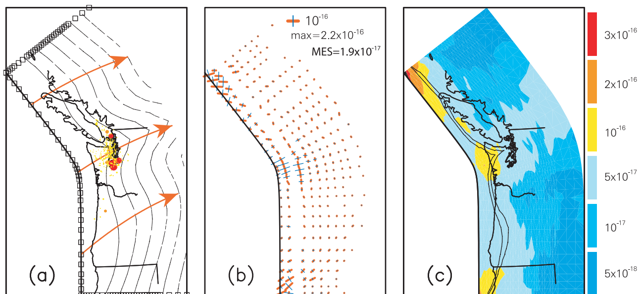
FIGURE 3: The variable-dip experiment showing results of the full inversion involving both the flow field and the slab geometry (see captions for Figure 2) for a power-law rheology ( n=10^6 ). The 10^\circ and 12^\circ iso-dip contours of the slab dip shown in panel c, come onshore under the Olympic Mountains, providing a possible explanation for the existence and location of this thick accretionary prism as explained in the text. The mean effective strain rate (MES) for power-law rheology is 2 \times 10^{-17} \text{ s}^{-1} .
