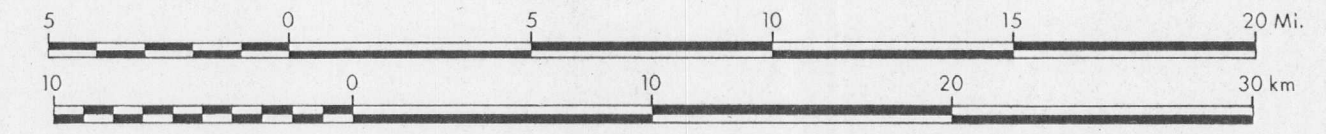
FIGURE 21 TOTAL SALINITY MAP OF THE BIRDBEAR FORMATION INTERVAL 20,000 ppm of TDS
