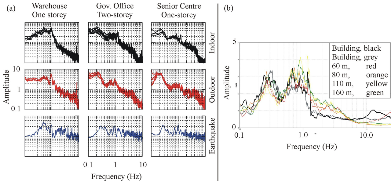
Figure 6. (a) Comparison of indoor and outdoor (within 50 m) microtremor and earthquake h/v spectral ratios at three strong-motion instrument locations in greater Vancouver demonstrate minor structural influence. Log-log plots. (b) Microtremor h/v spectral ratios 0 to 160 m distant of a 14-storey building are consistent. Log-linear plot.
