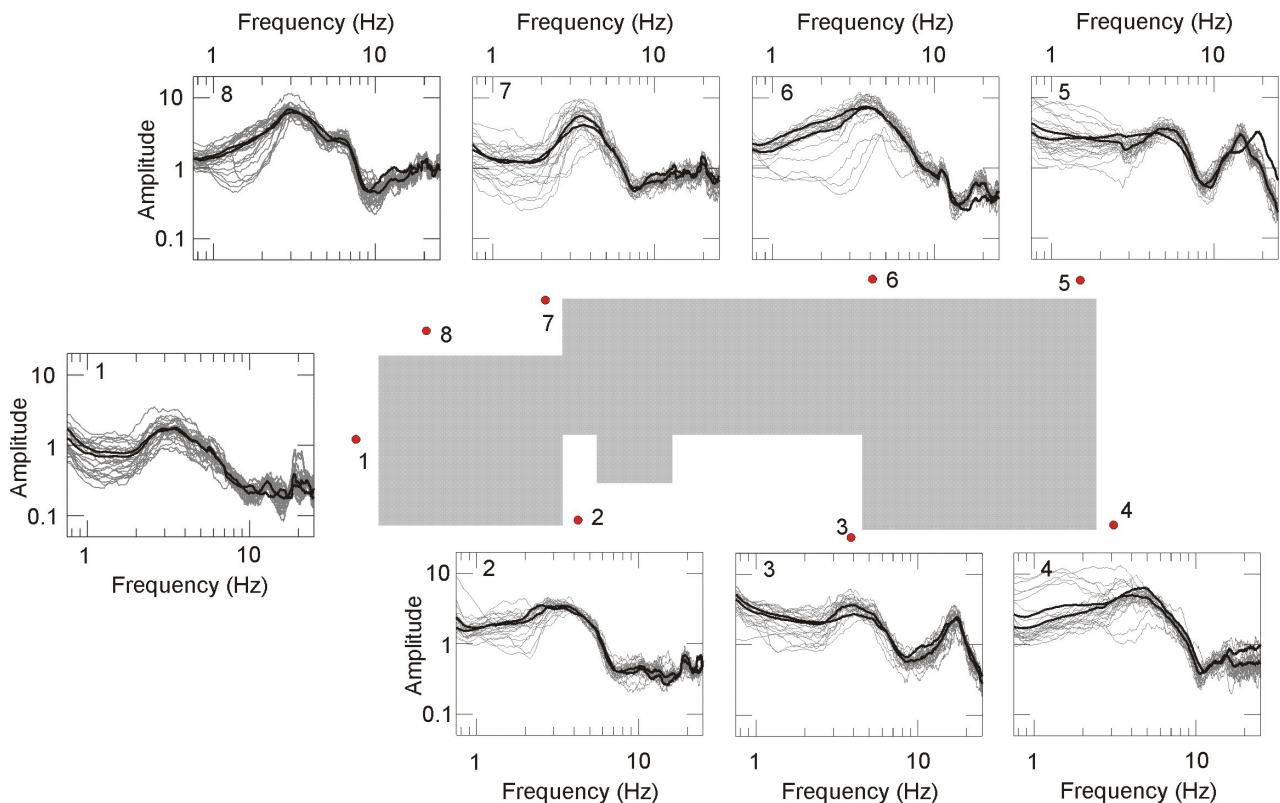
Figure 3. Microtremor site response at 8 sites surrounding a greater Victoria school building. The peak amplification shifts to lower frequency (longer period) with an increase of soft amplifying material and/or a decrease in average shear-wave velocity (i.e. the peak shifts towards the left). Log-log plots.
