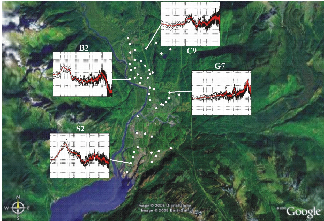
Figure 5. Google Earth aerial image of the 50 microtremor recording sites along a 10-km stretch of the Sea-to-Sky Highway that links Vancouver with Whistler. Log-log plots with frequency on the horizontal axis from 0.1 to 20 Hz (0.05 to 10 s) and h/v ratio amplitude on the vertical axis from 0.1 to 20.
