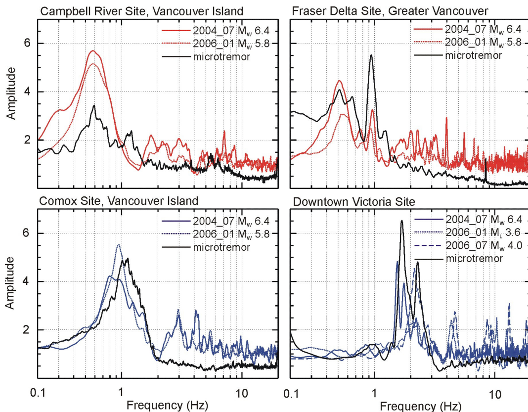
Figure 2. Comparison of the h/v spectral ratio from up to four weak-motion earthquakes and microtremors at four sites across SW British Columbia. Log-linear plots.
