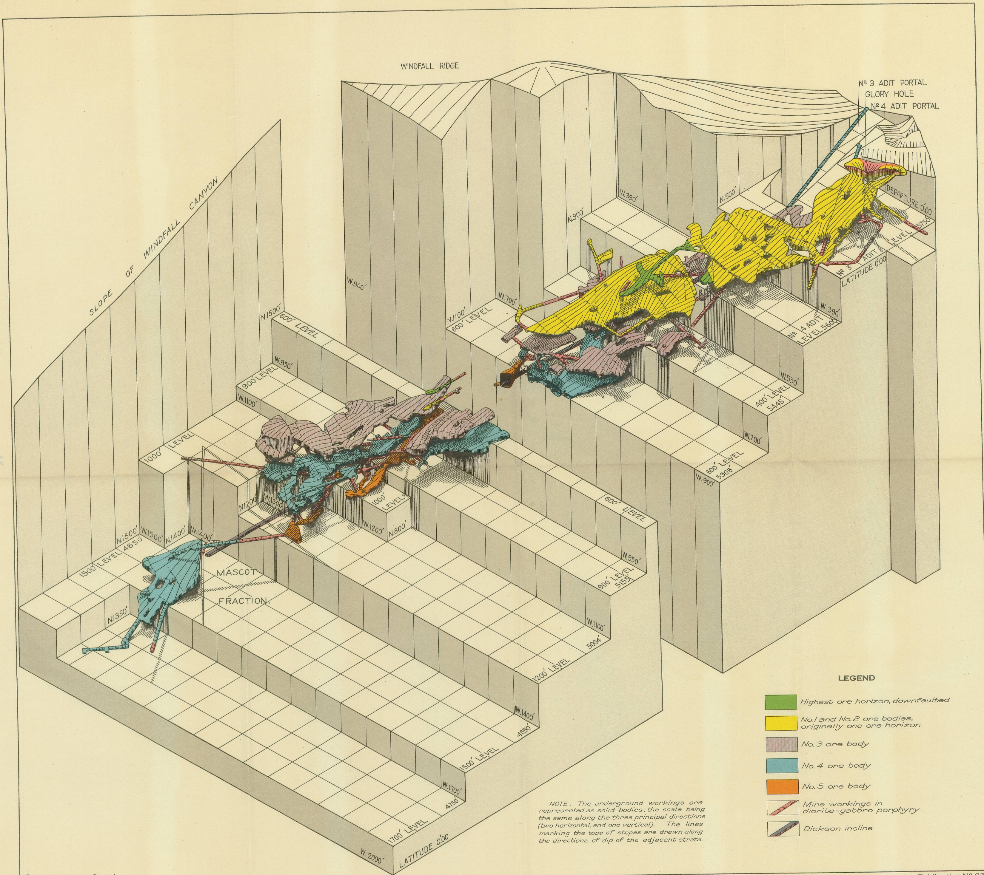
Figure 16 ISOMETRIC DIAGRAM OF THE UNDERGROUND WORKINGS OF NICKEL PLATE MINE, (NEAR HEDLEY), BRITISH COLUMBIA.
