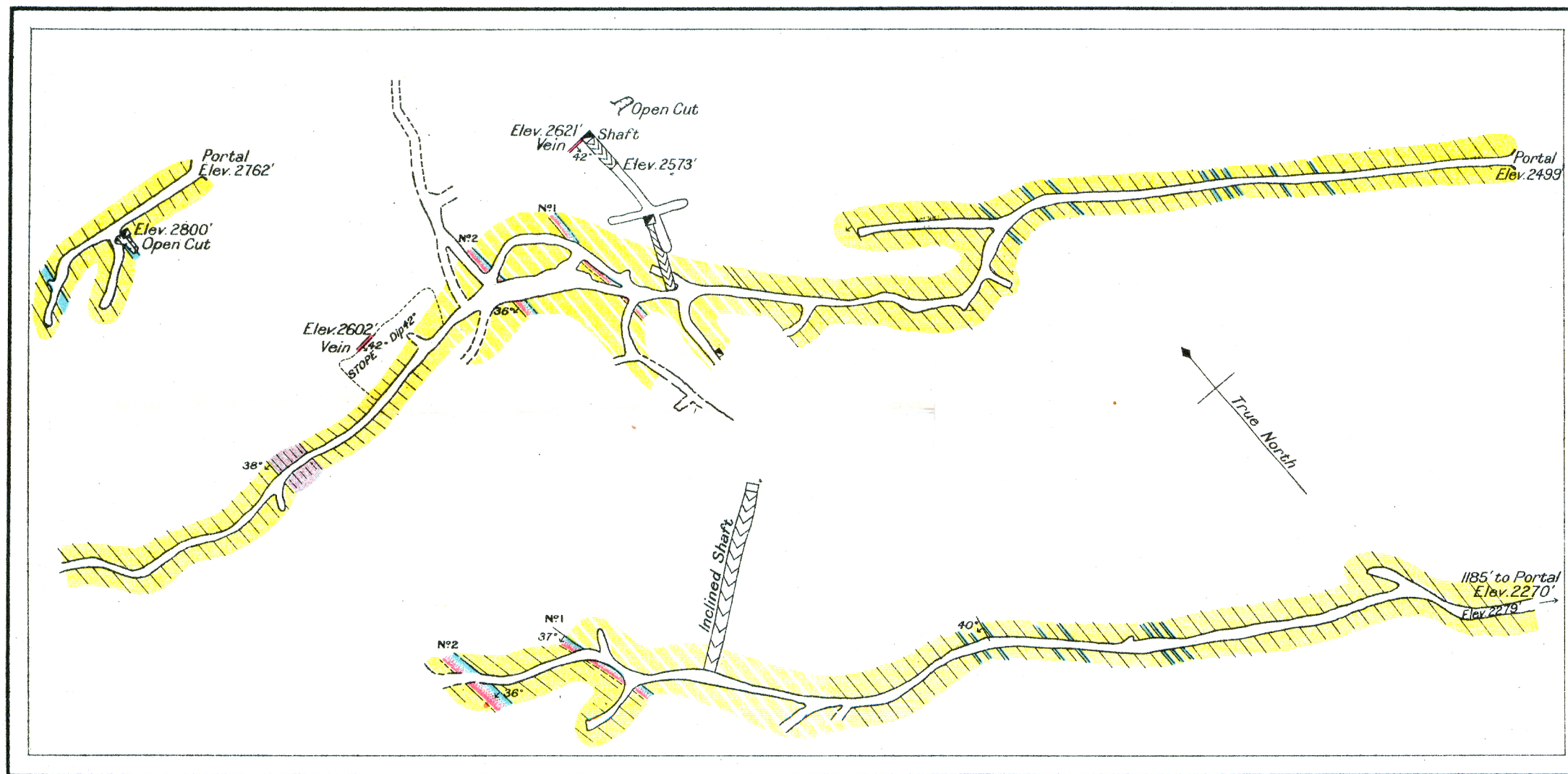
Diagram showing geology of the underground workings of the Florence Silver Mining Company, Ainsworth Mining Camp, Kootenay District, British Columbia.
