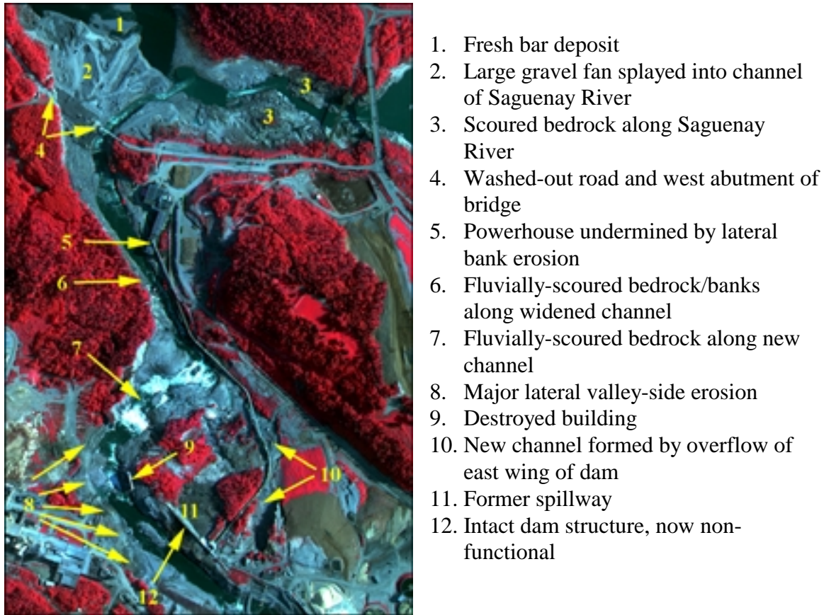
Figure 5. Geological interpretation by Dr. Greg Brooks and Dr. Ted Lawrence of the Geological Survey of Canada.
