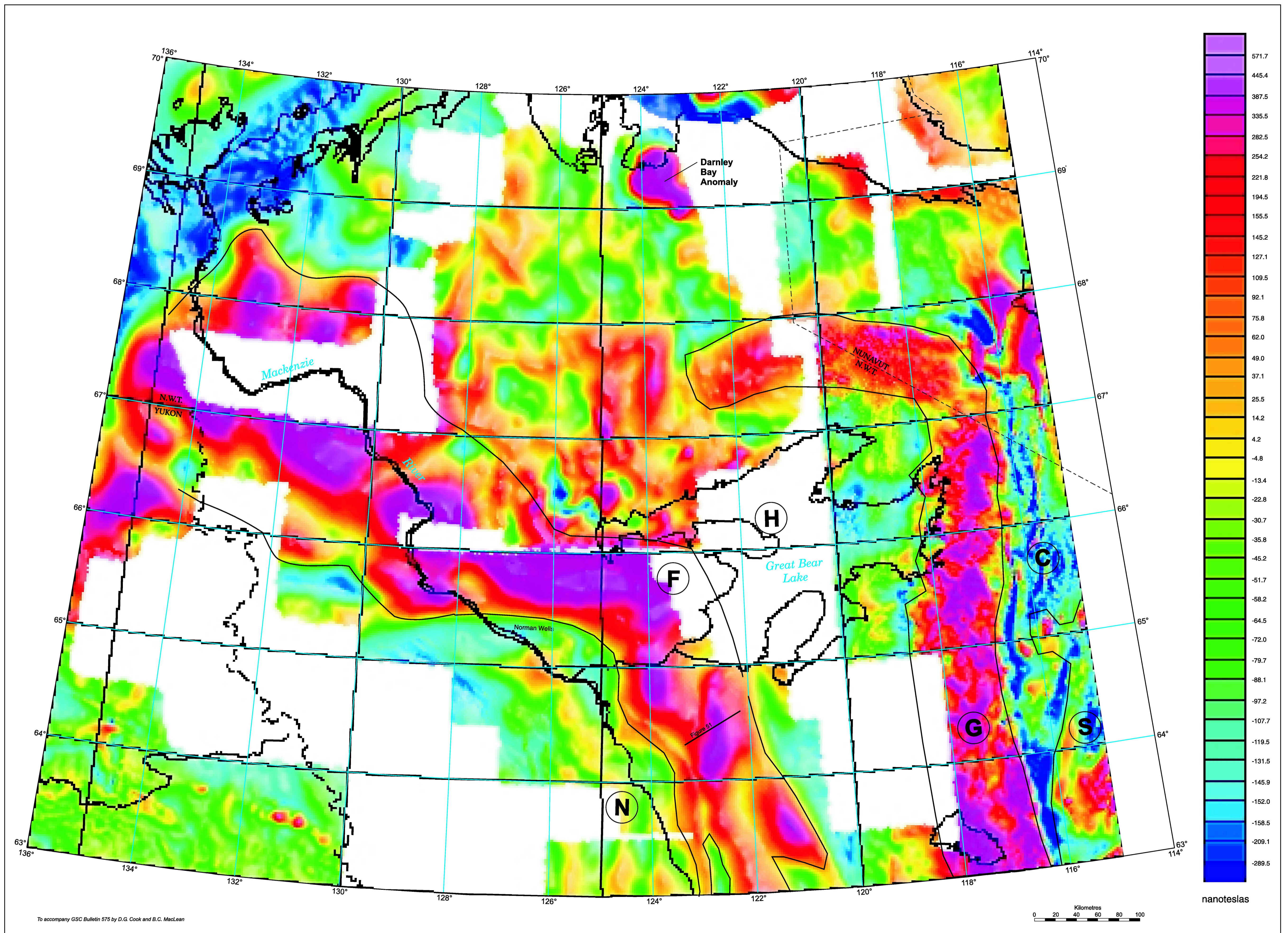
Figure 5. Total field aeromagnetic map (data from Continental Geoscience Division, Geological Survey of Canada). Basement terrane boundaries and age limits are after Ross (1991). N, Nahanni (age unknown); F, Fort Simpson (1.79–2.02 Ga); H, Hottah (1.85–2.38 Ga); G, Great Bear (1.79–2.02 Ga); C, Coronation (1.85–2.38 Ga); S, Slave (2.6–3.9 Ga).
