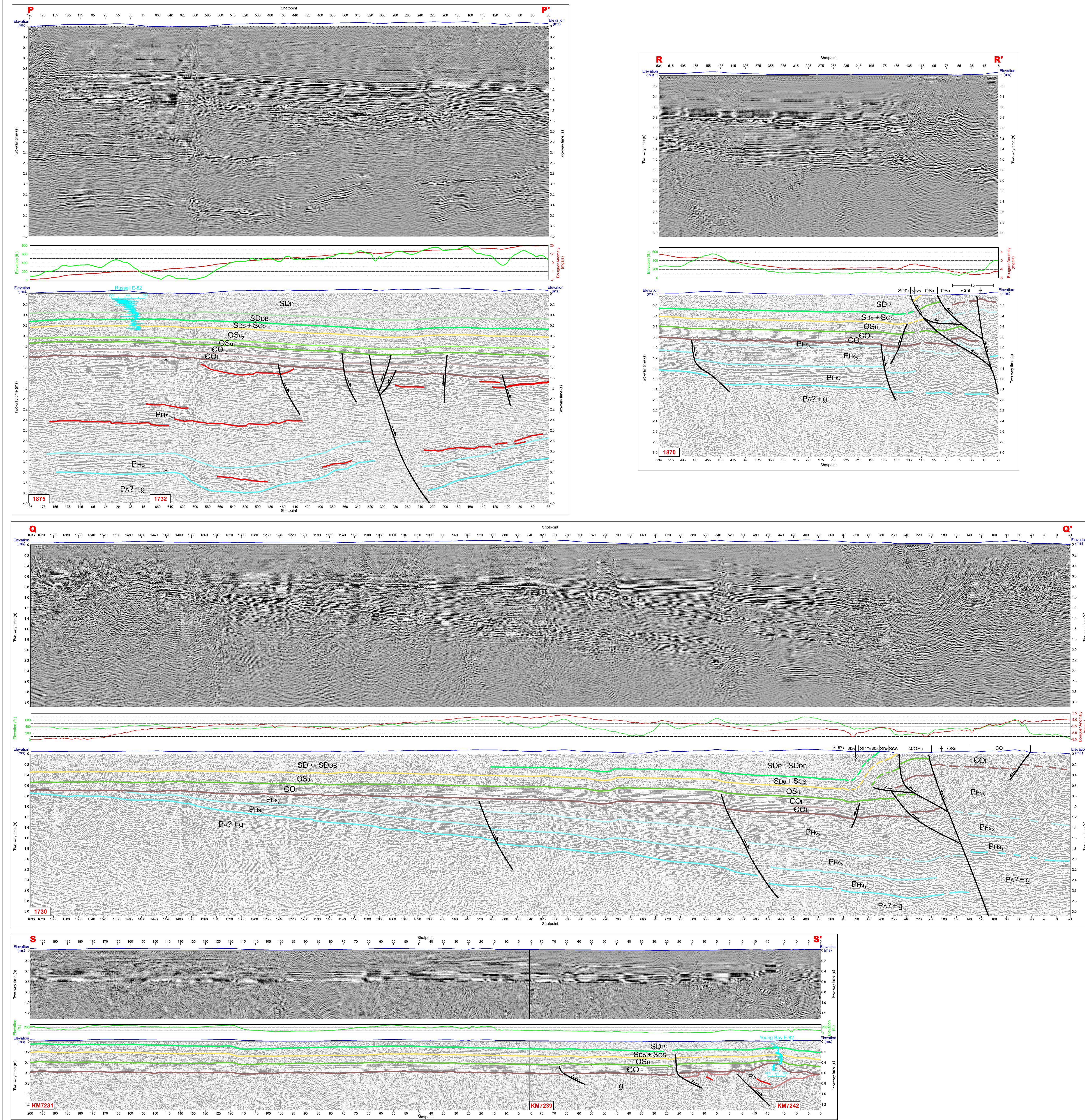
Figure 20. Seismic structure cross-sections.
