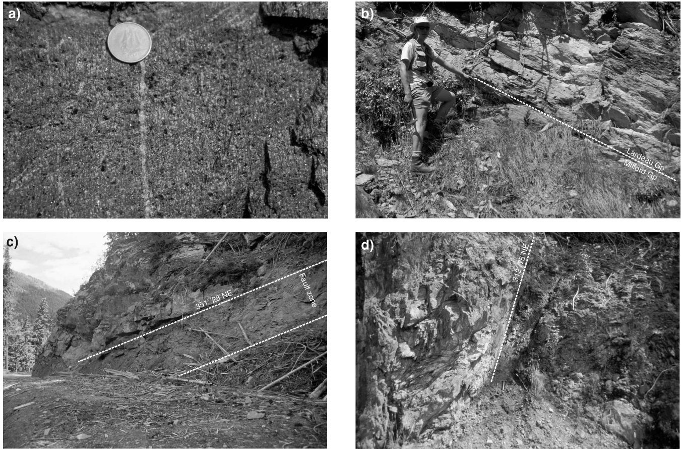
Figure 3. a) Natural outcrop surface of part of the Broadview Formation (Lardeau Group) showing abundant black quartz clasts. Coin is about 1 cm across. b) Unconformity (dashed line) between limestone of the Milford Group and underlying green phyllite of the Lardeau Group. This exposure represents an overturned limb of a tight southeast-verging fold. Dashed line highlights the unconformity. View looking to the northwest. c) Cataclastic zone on the northern flank of the southern Mesozoic outlier. Fault zone is about 2–3 m thick. Dashed lines define the faulted zone. View looking to the northeast. d) Discrete and brittle fault plane in a cataclastic zone east of Arrow Park. Dashed line represent the orientation of the discrete fault plane. View looking to the southeast. A hammer (40 cm) is visible at the base of the rock face.
