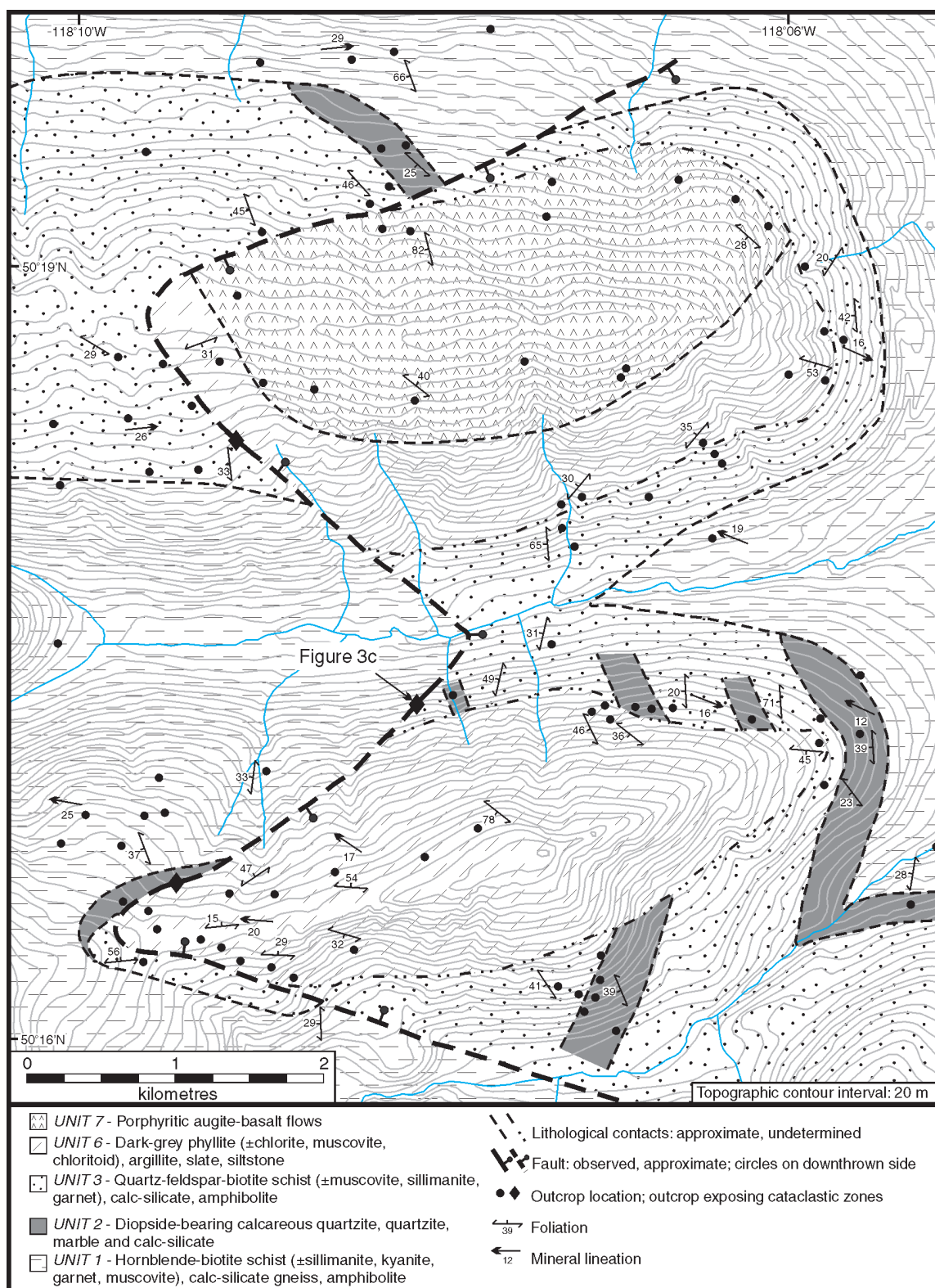
Figure 2. Geological map of two Mesozoic outliers west of Mosquito Lake (see Fig. 1 for location). Numbers refer to units described in the text.
