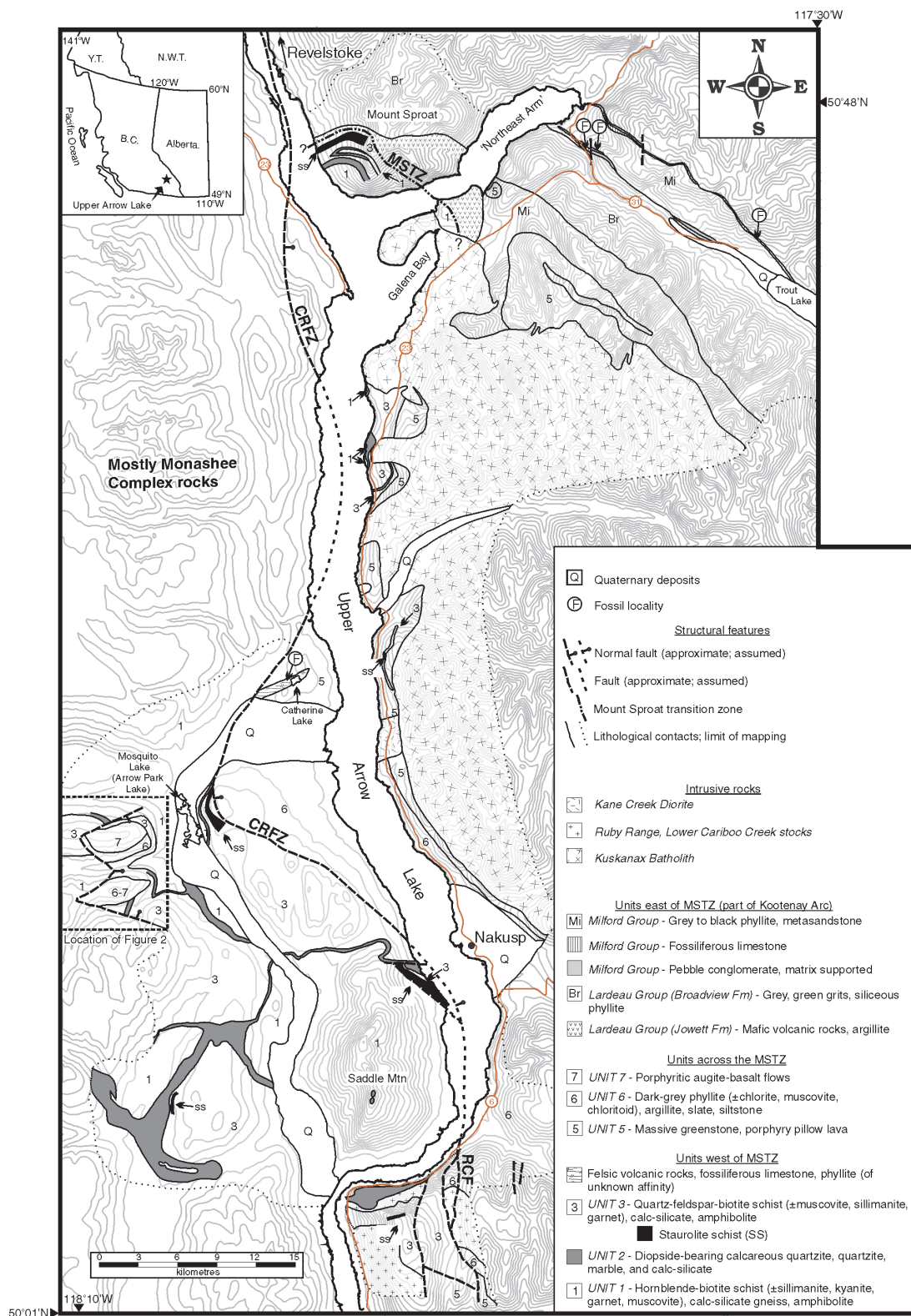
Figure 1. Geology of the Upper Arrow Lake area. CRFZ, Columbia River fault zone; RCF, Rodd Creek Fault; MSTZ, Mount Sproat transition zone. Inset: Location map of the Upper Arrow Lake area. Topographic contours from Canada NTS 1:250 000 scale Vernon and Lardeau maps.
