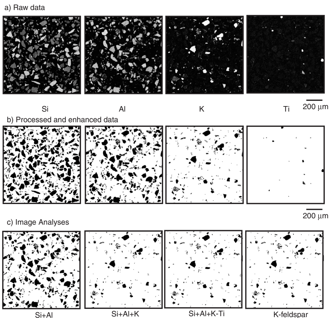
Figure 2. Scanning electron microscope photomicrographs of a) raw EDS maps for Si, Al, K, and Ti; b) maps of the same elements after setting the threshold, converting into binary images, and applying a cutoff value to eliminate background noise; c) maps showing how K-feldspar is derived. The first image in c) is the result of adding overlapping areas from the Si and Al maps of b) . The Si+Al +K map of c) is derived by adding the overlapping areas from the Si+Al map of c) to the K map of b) . The third image of c) , Si+Al+K-Ti, illustrates the areas of Ti to be subtracted in grey. Subtracting the Ti file helps reduce the possibility of the final map containing grains of biotite. The field of view is representative of the area examined for feature image analysis and X-ray mapping.
