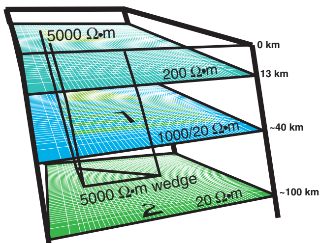
Figure 2. Three-dimensional forward model, perspective view. Features 1 and 2 from the text are identified.
