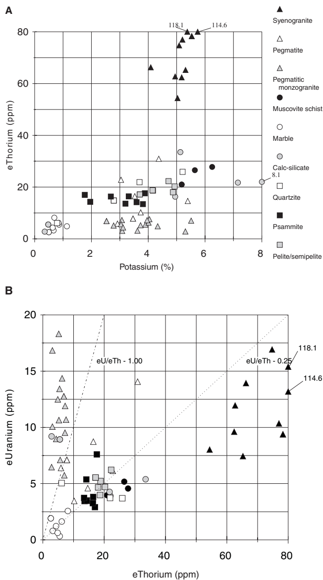
Figure 4. Radioactive element plots for 64 ground gamma-ray spectrometry measurements from the Flint Lake area, central Baffin Island.
