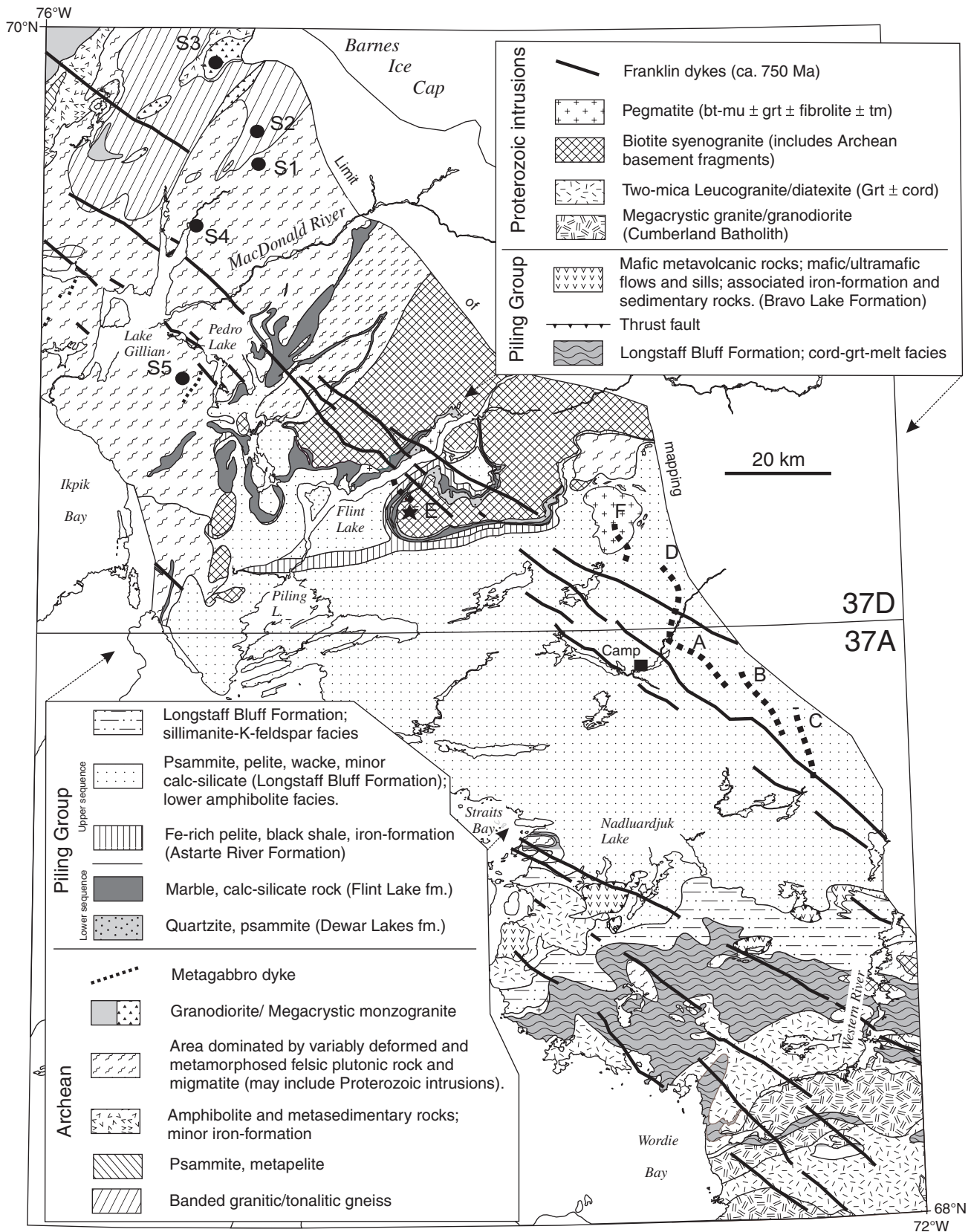
Figure 2. Simplified geological map of part of the Foxtie Fold Belt, central Baffin Island from Corrigan et al. (2001) showing the location of gamma-ray spectrometry traverses (A–F) and sites (S1–S5); bt=biotite, mu=muscovite, grt=garnet, tm=tremolite, cord=cordierite.
