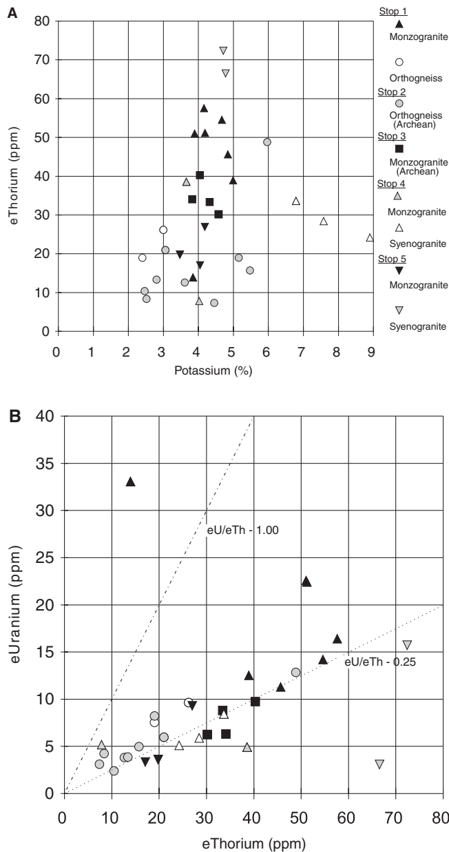
Figure 5. Radioactive element plots for 32 ground gamma-ray spectrometry measurements for granitic and gneissic lithologies from the MacDonald River and Drewry River areas, central Baffin Island.
