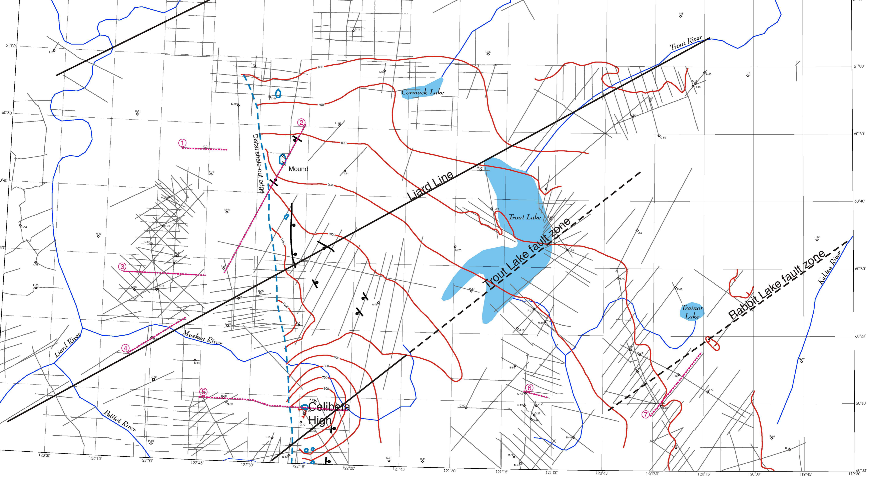
Figure 1, Map F Seismic time structure map: Top of Jean Marie Member, Redknife Formation Contour Interval: 100 ms two-way-time; Datum = 600 m asl Normal fault Reverse fault Monocline Well location Seismic track Seismic illustration 0 5 10 Kilometres Lambert Conformal Projection: 60.5° / 61.5° 120°
