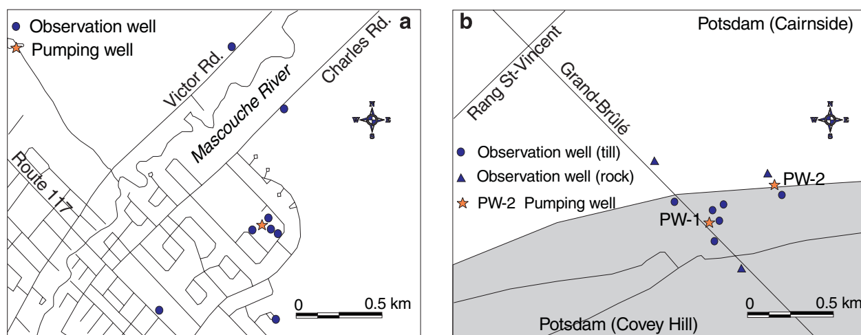
Figure 5. a) Saint-Janvier detailed aquifer test study. b) Saint-Benoît detailed aquifer test study.
