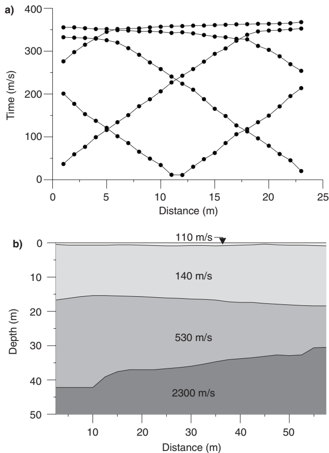
Figure 5. a ) Travel-time versus distance diagram for first-arrival refractions compiled from five records acquired at site 26 (Fig. 1). b ) Shear-wave velocity model resulting from application of the seismic refraction method.
