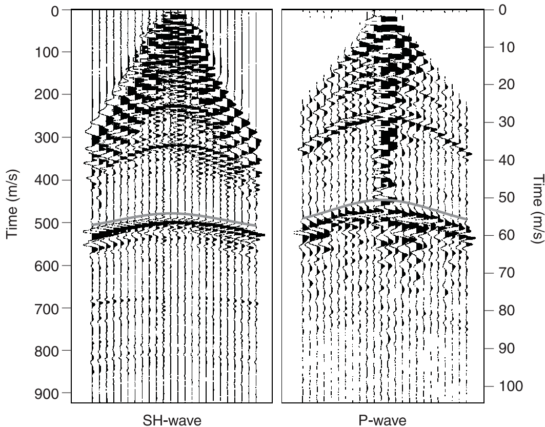
Figure 3. Comparison between the central spread of site 35 (Fig. 1) from SH-wave (left) and P-wave (right) reflection surveys. The grey line indicates reflection from bedrock. The SH-wave shot gather is displayed without any previous filtering. The P-wave record has been filtered using a Butterworth filter with frequency corners 200-300-800-1000 Hz to remove the Rayleigh wave interference. The vertical scales differ between the P-wave and SH-wave shot gathers allowing direct correlation of events in both records.
