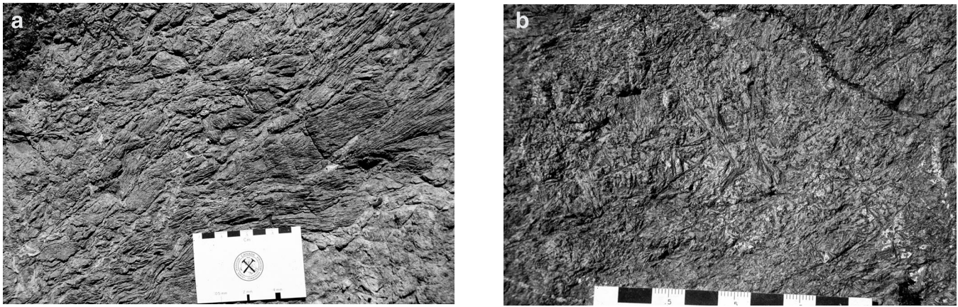
Figure 3. Spinifex-textured ultramafic rocks of the Red Lake belt. a) bladed olivine komatiite, Balmer assemblage, Golden Arm; b) acicular clinopyroxene komatiitic basalt, Ball assemblage, Miles Creek.
