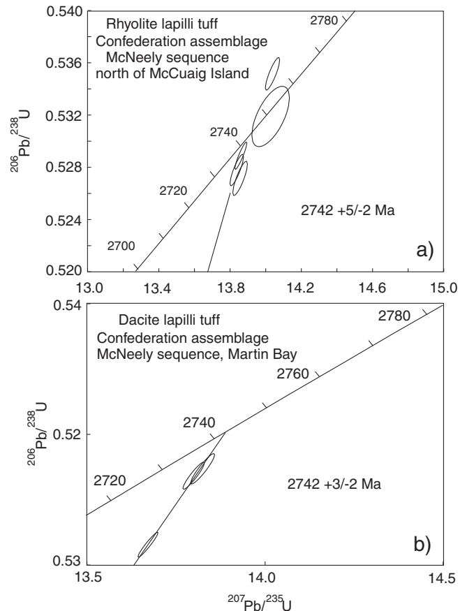
Figure 9. Uranium-lead ages of the McNeely sequence, Confederation assemblage. a) U-Pb concordia diagram of rhyolite tuff from central Red Lake (UTM 15 441671E, 5660288N), and b) U-Pb concordia diagram of dacite lapilli tuff, Martin Bay (UTM 15 427507E, 5655386N).
