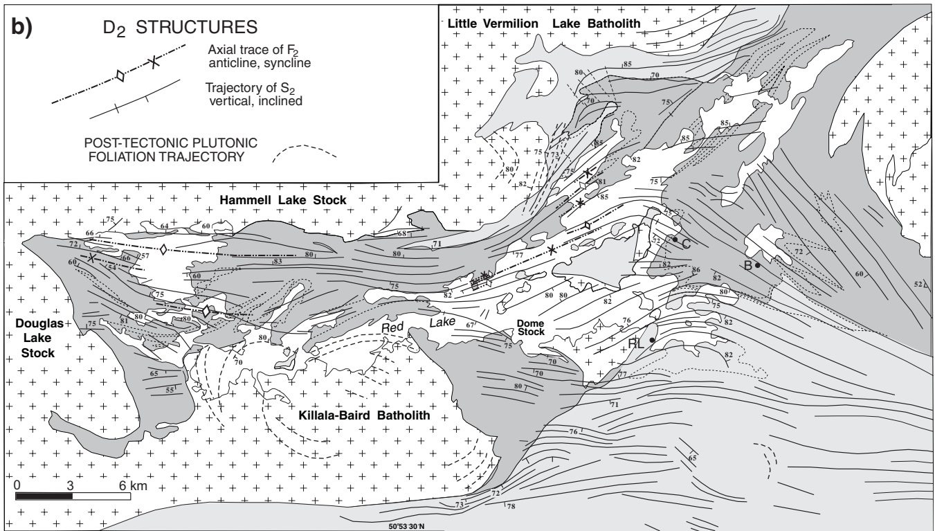
Figure 11. Structural data from the Red Lake belt. a) D 1 structures. b) D 2 structures and post-tectonic granitoid fabrics. B = Balmertown; C = Cochenour; RL = Red Lake
