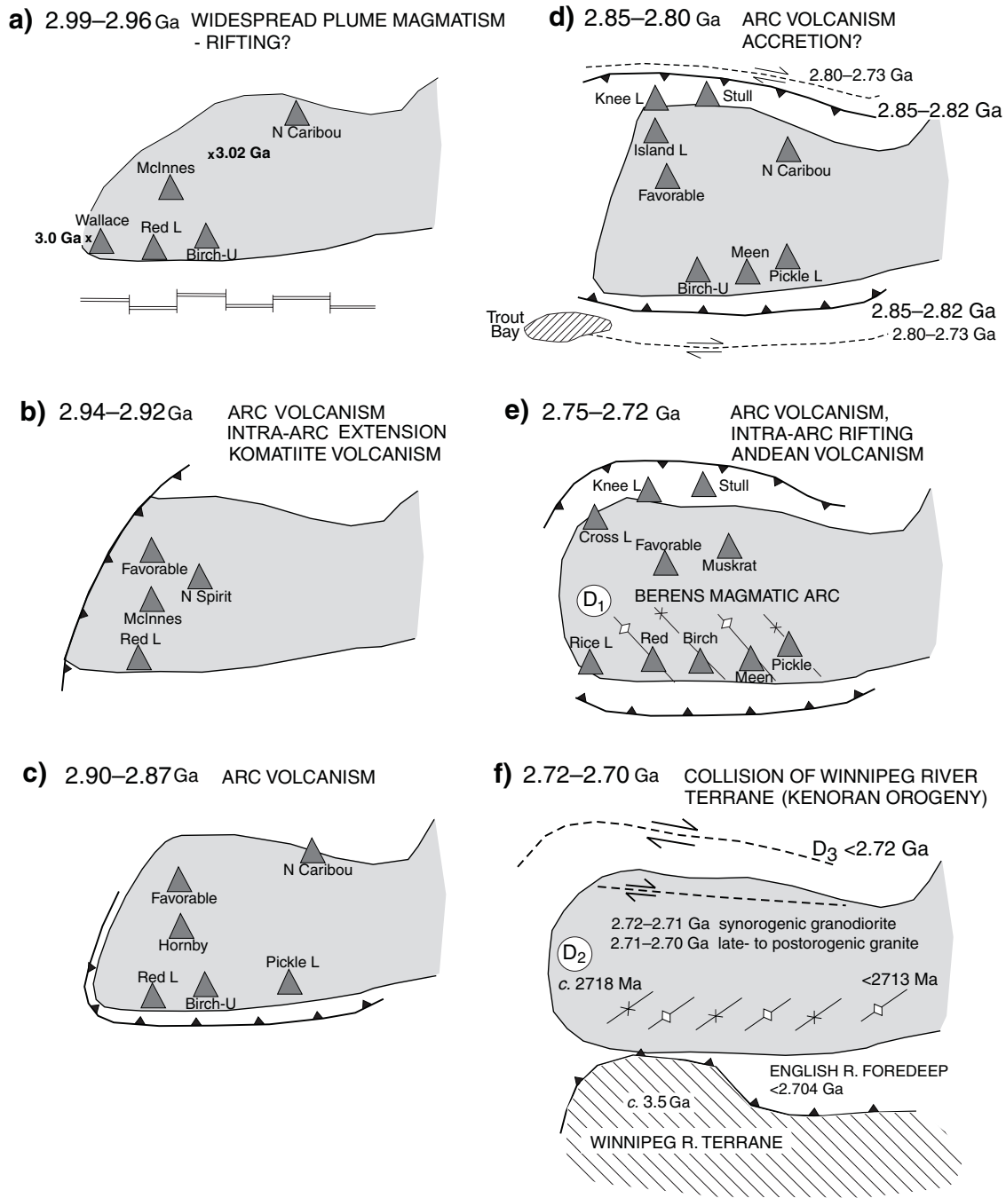
Figure 13. Geodynamic setting of the Red Lake greenstone belt and evolution of the North Caribou terrane. a) Plume-related magmatism on 3 Ga North Caribou protocraton; b) arc magmatism and intra-arc extension leading to komatiite eruption; c) arc magmatism encompasses the southern North Caribou terrane; d) arc volcanism and accretion of oceanic rocks of the Trout Bay assemblage; magmatic quiescence at this time may reflect a change from arc volcanism to transpression; e) Neoproterozoic arc volcanism and intra-arc rifting reflecting subduction along the northern and southern margins; a shift from extensional to compressional arc magmatism at 2.73 Ga coincides with the development of the Andean-style Berens River arc, D1 deformation and uplift; f) 2.72 to 2.70 Ga diachronous collision of the Winnipeg River terrane.
