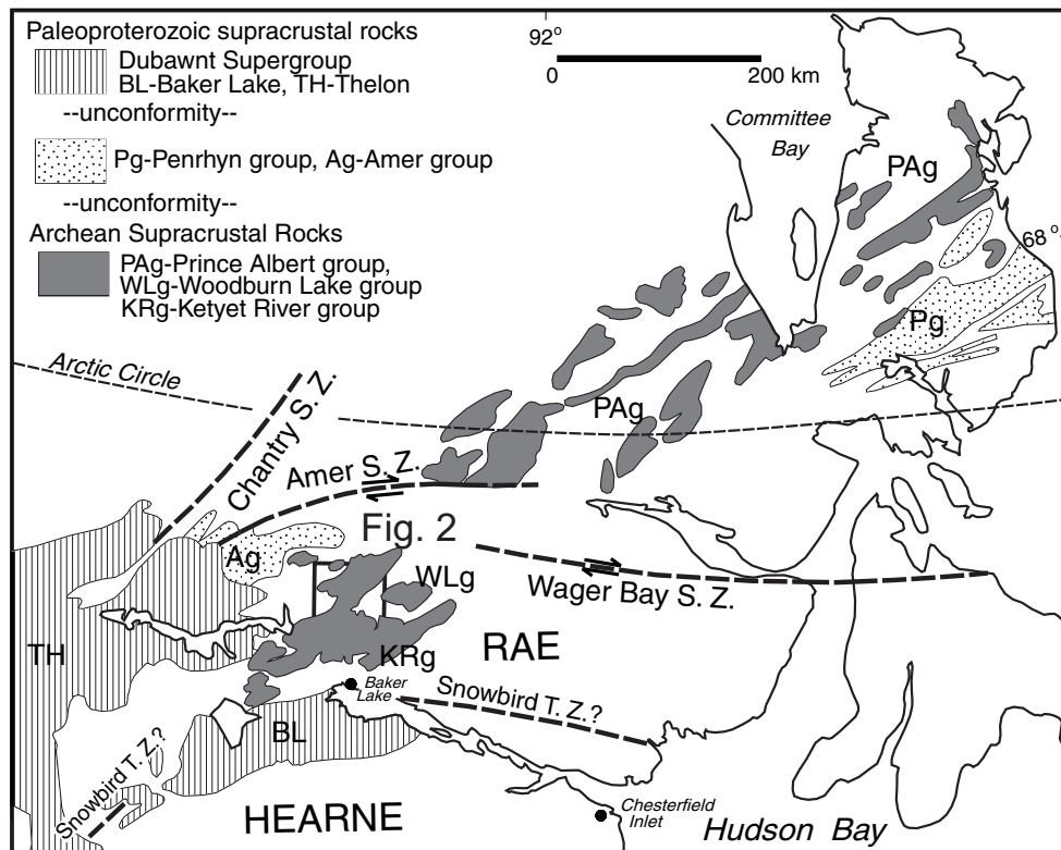
Figure 1. Regional geological sketch map of the western Churchill Province, showing the distribution of Archean supracrustal rocks in the Woodburn Lake group (WLg), the Prince Albert group (PAg), and the Ketyet River group (KRg) relative to the Paleoproterozoic suites of the region (Zaleski et al., 1997b).
