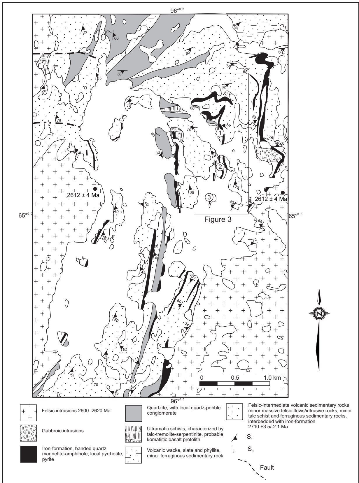
Figure 2. Simplified geological map of the Woodburn Lake group in the Meadowbank area (Zaleski et al., 1997a, 1999a). Circled numbers: 1. North Portage deposit, 2. Third Portage deposit, 3. Goose Island deposit. The Bay Zone deposit is immediately southwest of Third Portage.
