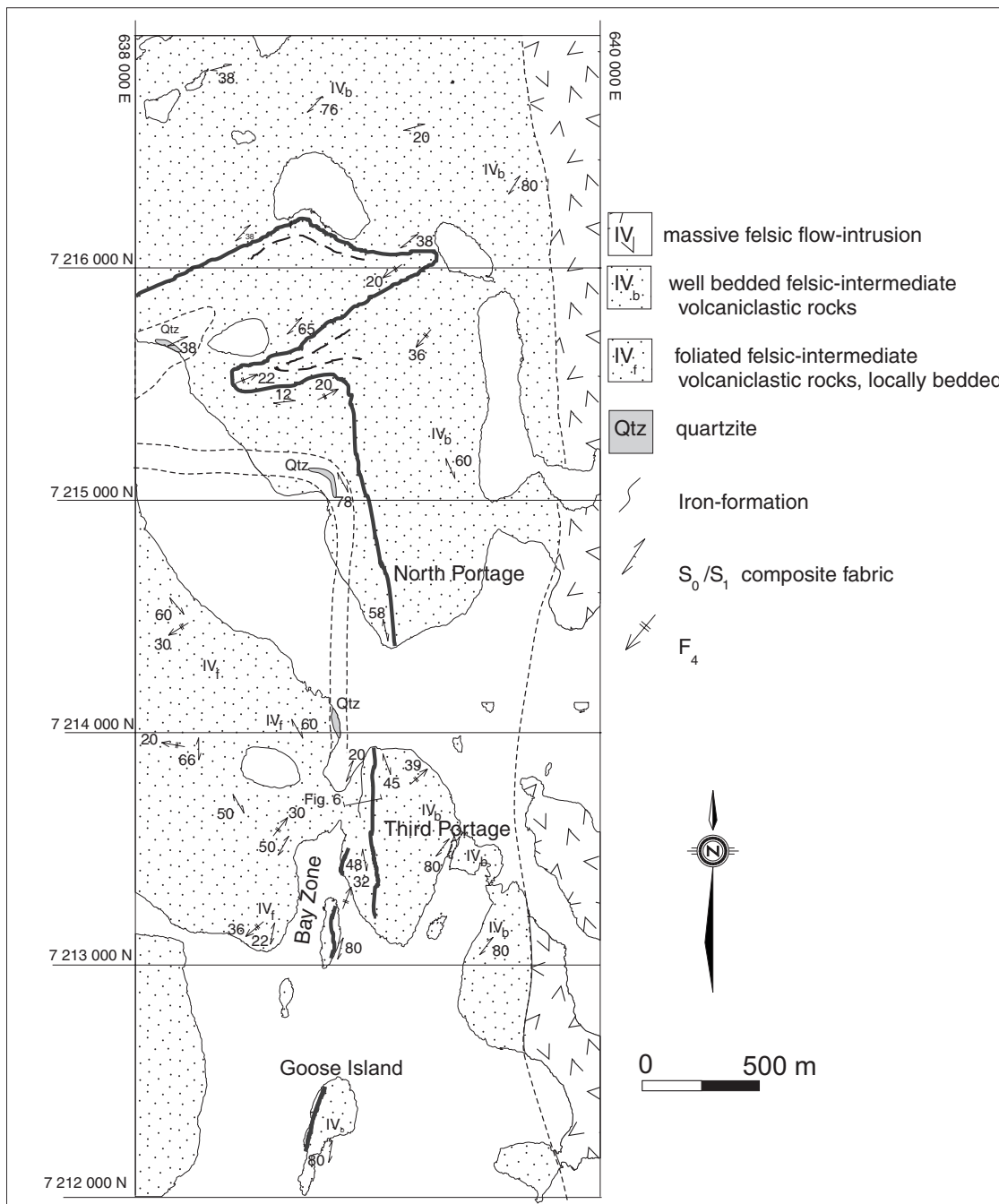
Figure 3. Simplified geological map of the Meadowbank deposits showing the distribution of the rock types and tectonic fabrics. Cross-section in Figure 6 is shown in the Third Portage deposit.
