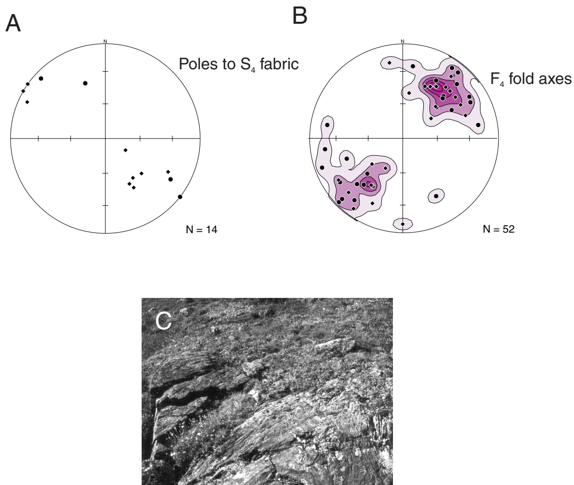
Figure 5. Stereonet plot of poles to S_4 fabric (A) and measured F_4 axes (B). For both plots, circles represent data from the North Portage deposit and diamonds from the Third Portage deposit. C) Photograph of F_4 folds from the North Portage area.
