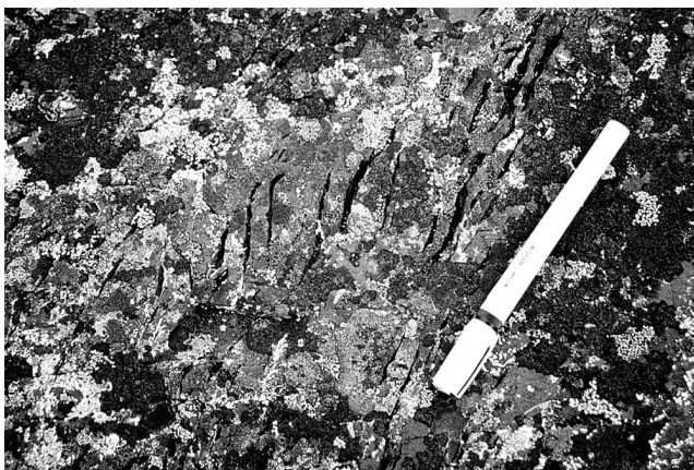
Figure 11. Tension gashes show progressive sinistral rotation, over a strain gradient leftward of the pen, from fractures trending approximately 040°. The pen is oriented at 048°. These are interpreted to be related to a regional set of sinistral strike-slip faults that trend about 040°.
