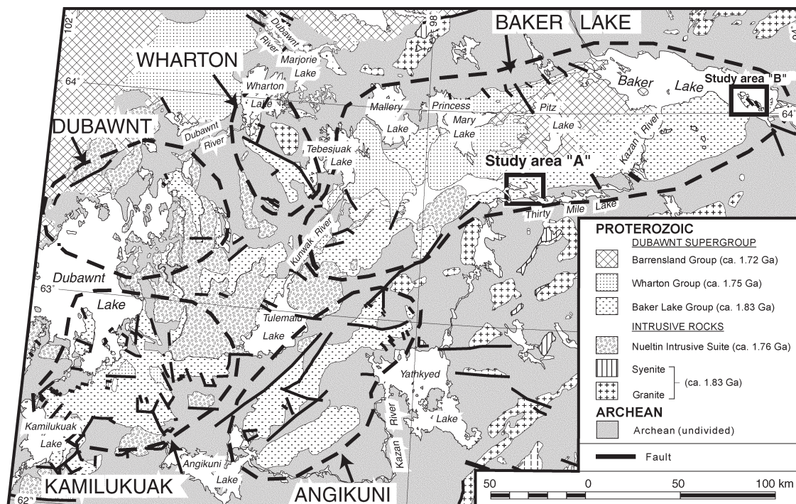
Figure 1. Geology of the Baker Lake Basin comprising the Baker Lake, Wharton, Dubawnt, Kamilukuak and Angikuni Sub-basins (after Donaldson, 1965; LeCheminant et al. 1979; Blake 1980), showing locations of study areas discussed in this report.
