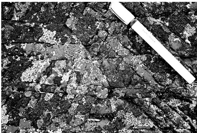
Figure 10. Three fracture sets, trending about 100°, 040°, and 40°, are developed. The pen is oriented at 340°. The approximately 100° fracture set crosscuts the other fracture sets in the left-central part of the photograph.
