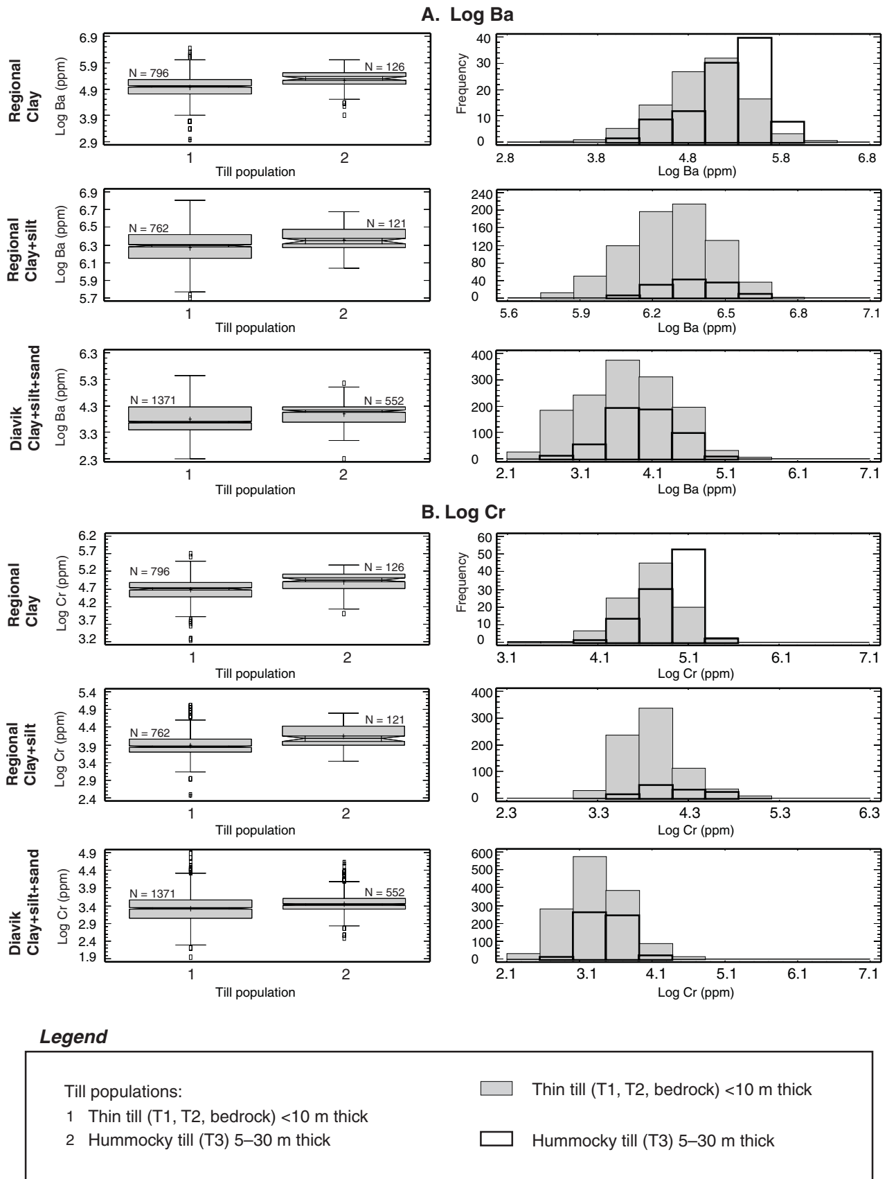
Figure 4. Comparison of Ba and Cr concentrations by till thickness, for each till size fraction. ‘Bedrock’ refers to till samples from areas of >75% bedrock exposure.
