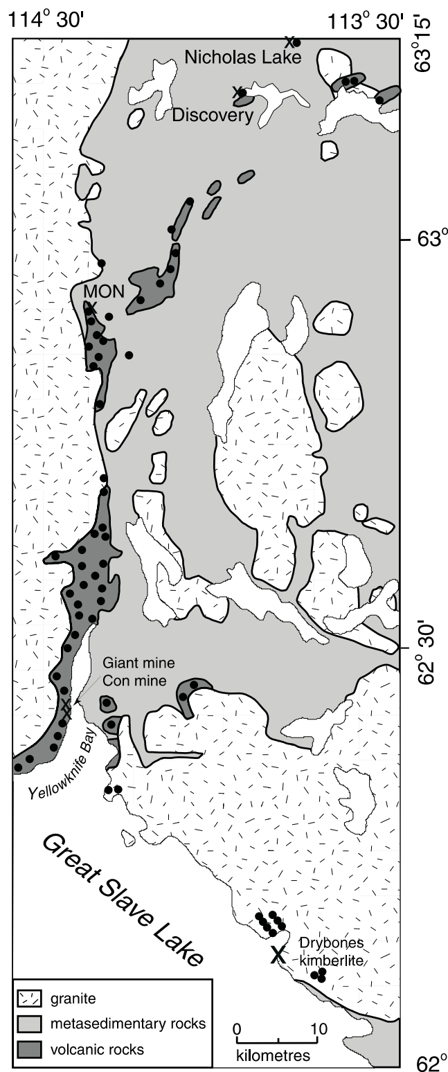
Figure 2. Location of sample sites (black dots) and generalized bedrock geology with selected mineral deposits; modified from Jolliffe (1942), Henderson (1985), and Stuble (1997).
