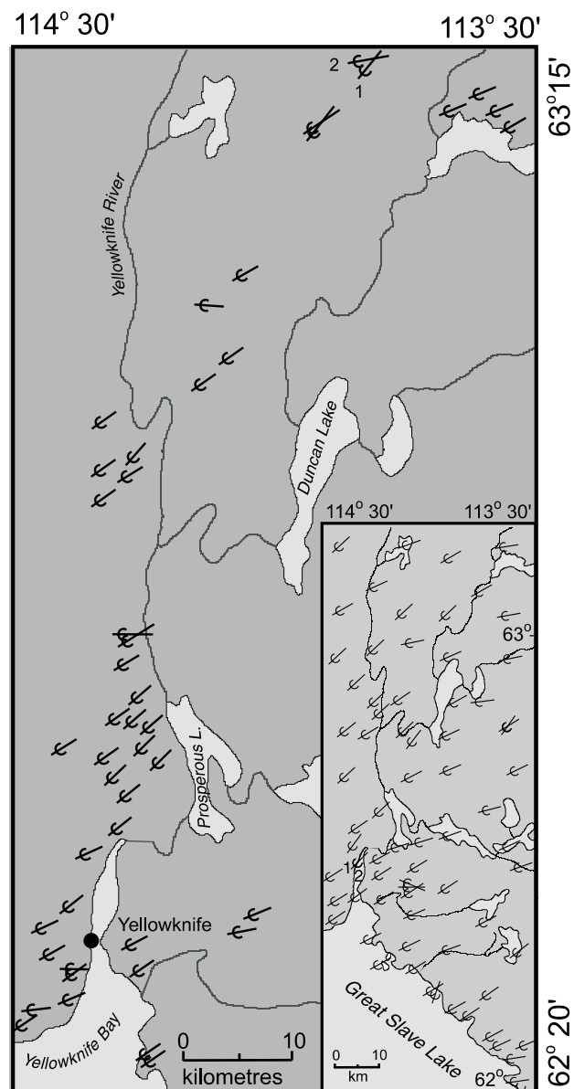
Figure 4. Detailed ice-flow summary diagram over the Yellowknife Greenstone Belt; 1 = oldest, 2 = youngest. Inset map shows regional ice flow.
