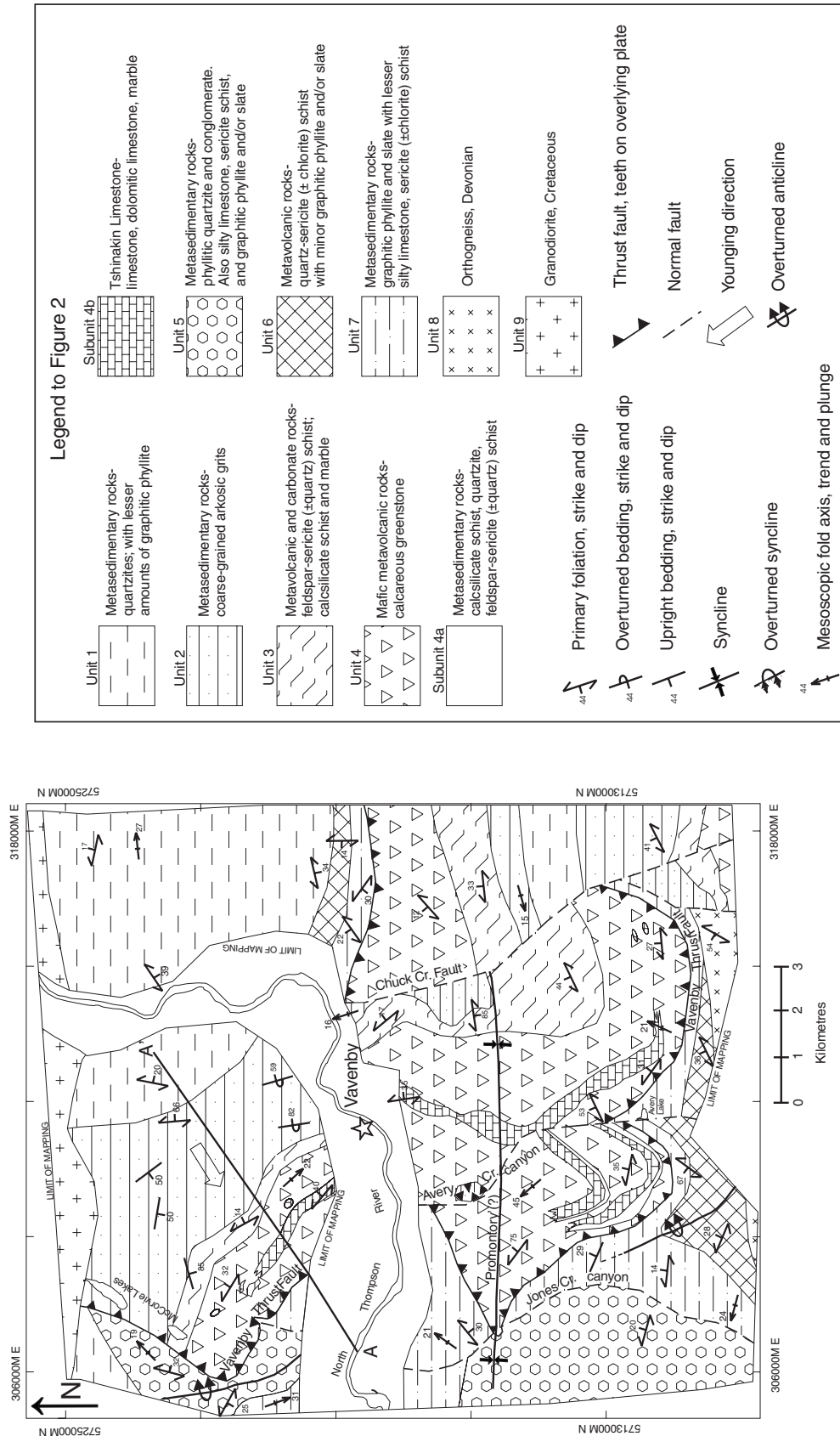
Figure 2. Preliminary geological map of the Vavenby area (this study).
