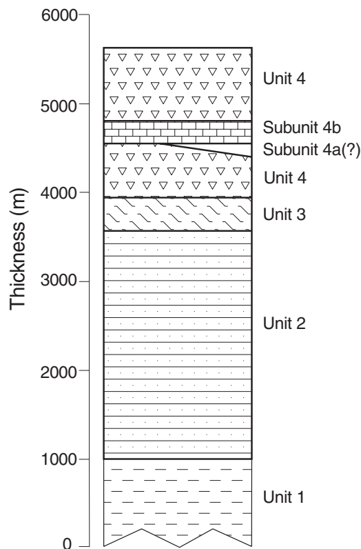
Figure 3. Schematic stratigraphic section of the early Cambrian (and possible older) succession of the Eagle Bay Assemblage northwest of Vavenby.
