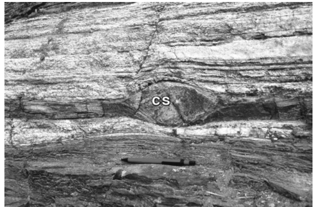
Figure 6. Calc-silicate (cs) pod within layered white marble and schist (unit 5). Pencil for scale.
