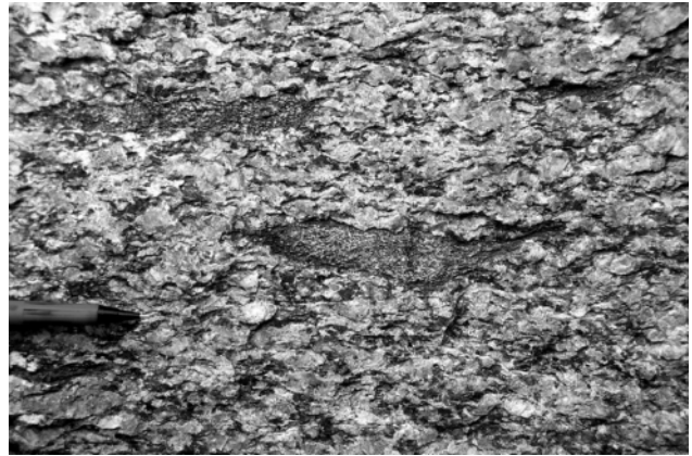
Figure 12. Metasedimentary xenoliths in coarse augen granite (unit 11). Pencil for scale.
