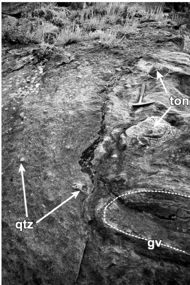
Figure 5. Deformed conglomerate (unit 2), dominated by quartz (qtz) pebbles, with rare tonalite (ton) boulders. Note folded granite vein (gv).
