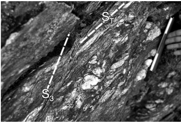
Figure 16. Steeply east-dipping, S_3 spaced crenulation cleavage (shear band geometry) overprints S_T , and decapitates isoclinal F_2 closures outlined in quartz veins in mica-quartz schist. Notebook is 20 cm long.
