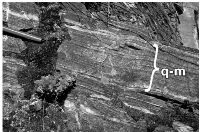
Figure 9. Finely laminated, statically recrystallized quartz-mylonite (q-m) layers in amphibolite schist (unit 6). Pencil for scale.
