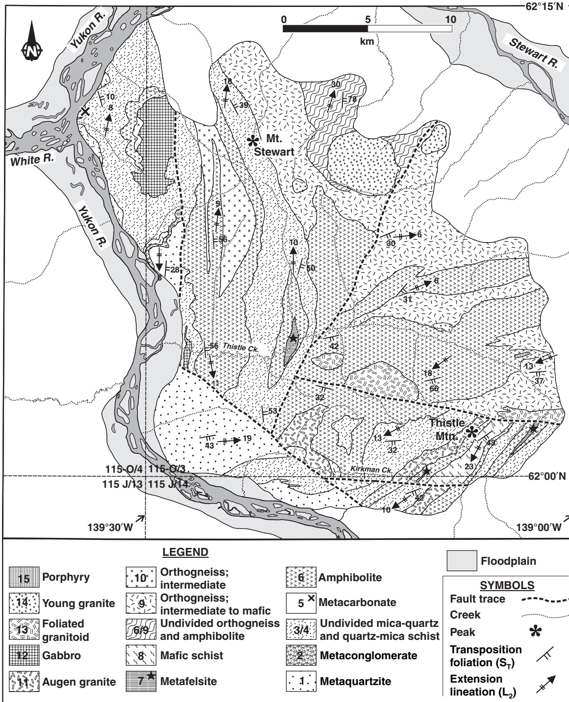
Figure 2. Simplified geological map of the Thistle Creek area.
