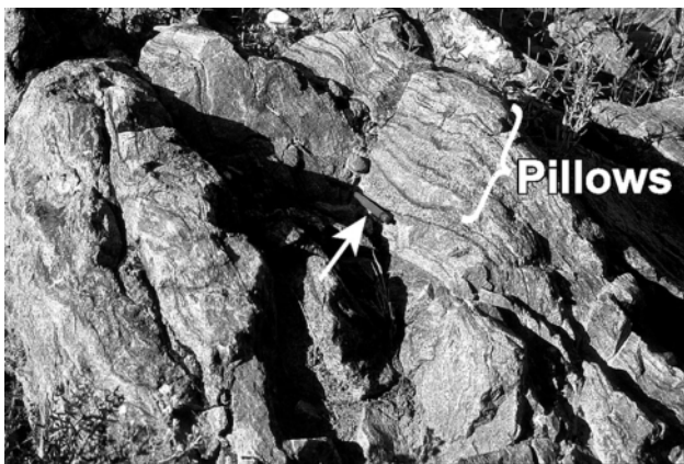
Figure 7. Layer of possible strongly flattened pillow selvages in a banded amphibolite (unit 6). Hornblende reaction halos are symmetrical about these features. Pencil for scale (arrow).
