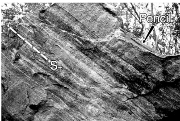
Figure 11. Typical banded appearance of heterogeneous, compositionally layered gneiss (unit 9) composed of diorite, tonalite and granodiorite. Pencil for scale.
