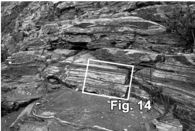
Figure 13. Planar, high-strain (protomylonitic) mixture of tonalite sheets in amphibolite. Pencil for scale (see Fig. 14).
