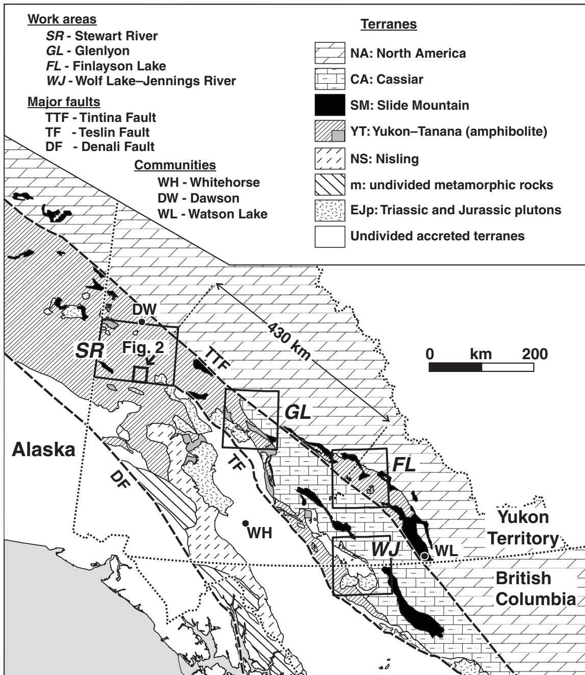
Figure 1. Location of the NATMAP project areas in Yukon Territory and northern British Columbia. Restoration of Cretaceous–Tertiary dextral offset of about 430 km (Dover, 1994) along Tintina Fault would place the Stewart River area in close proximity to the Finlayson Lake area. A project in southern British Columbia (not included on this figure) comprises the southern component of the NATMAP project (see Thompson et al., 2000 and references therein).
