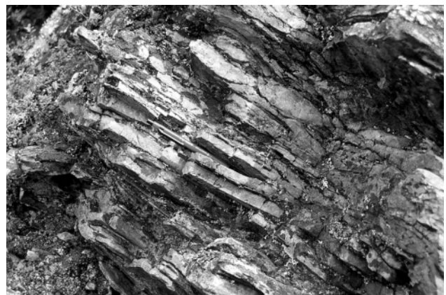
Figure 4. Rhythmically layered quartzite (unit 1), with thin laminations of semipelite. May represent recrystallized chert. Pencil for scale.
