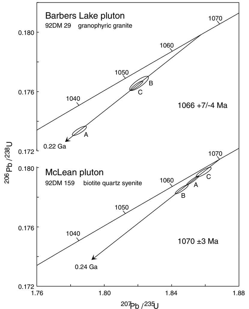
Figure 3. Uranium-lead concordia diagrams for granites from the Barbers Lake and McLean plutons, Sharbot Lake domain.
