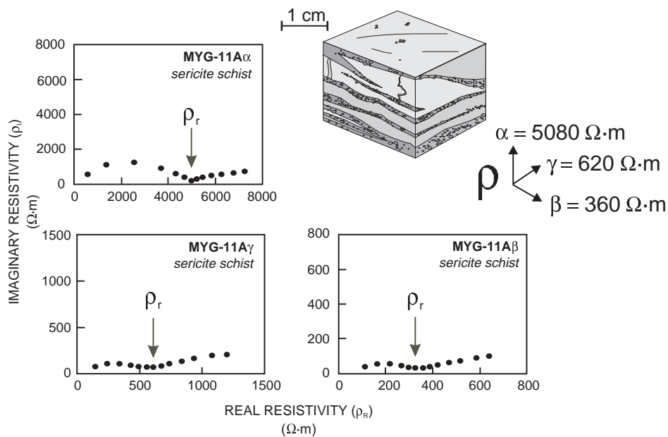
Figure 3. Visual description of a sericite schist sample (MYG-11A) with \rho_r values displayed for the three directions (5080, 360, and 620 \Omega \cdot m ) with an electrical anisotropy ( \lambda ) of 14:1 (Connell et al., 2000b), and the argon diagrams showing how the \rho_r values were determined.
