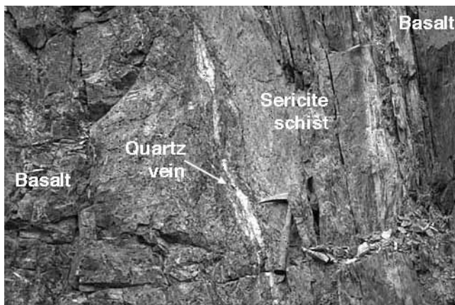
Figure 1. Photograph of a rock face displaying a typical gold-bearing quartz-ankerite vein, with sericite schist and chlorite schist alteration envelopes, all hosted in massive basalt (Giant mine, Northwest Territories). The samples used in this study were taken from positions along lines that traverse all of these four rock types.
