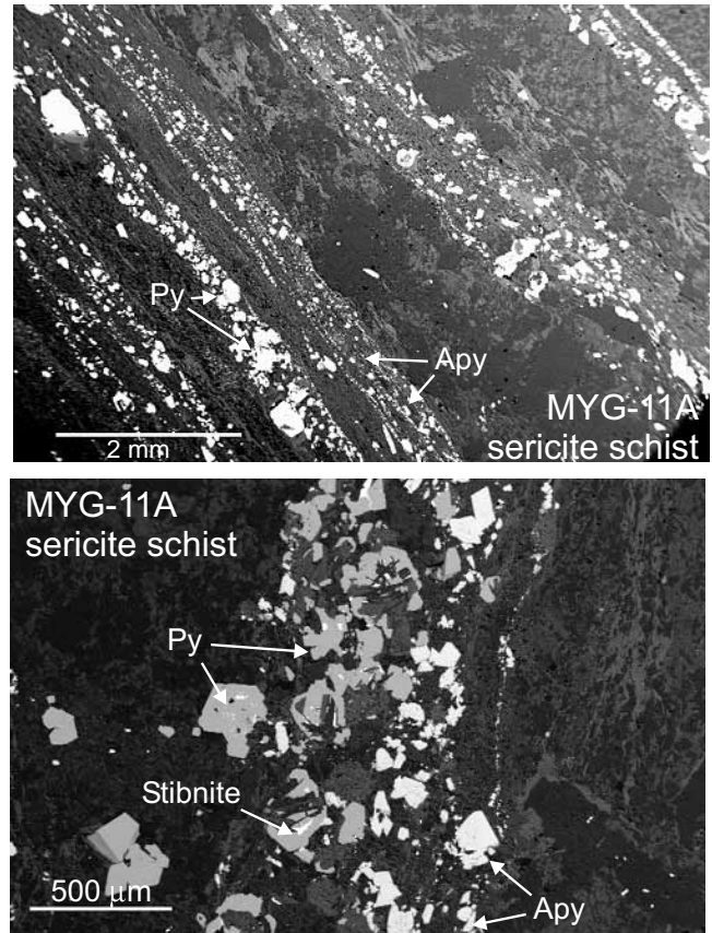
Figure 5. Scanning electron microscopy images of the sericite schist sample (MYG-11A), from the Giant mine (Northwest Territories), displaying sulphide-rich bands, which coincide with the low electrical resistivity ( \rho_r ) direction of the sample. The sulphide grains are generally euhedral in shape and show little grain-to-grain interconnectivity, resulting in intermediate \rho_r values (300–600 \Omega\cdot m ). Sulphide minerals include pyrite (Py), arsenopyrite (Apy), and stibnite.
