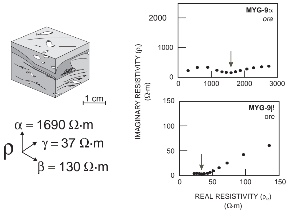
Figure 2. Visual description of an ore sample (MYG-9) with electrical resistivity ( \rho_r ) values displayed for the three directions (1690, 130, and 37 \Omega \cdot m ) with an electrical anisotropy ( \lambda ) of 46:1 (Connell et al., 2000b), and the argon diagrams showing how the \rho_r values were determined from the frequency spectrum of the complex electrical resistivity measurements.
