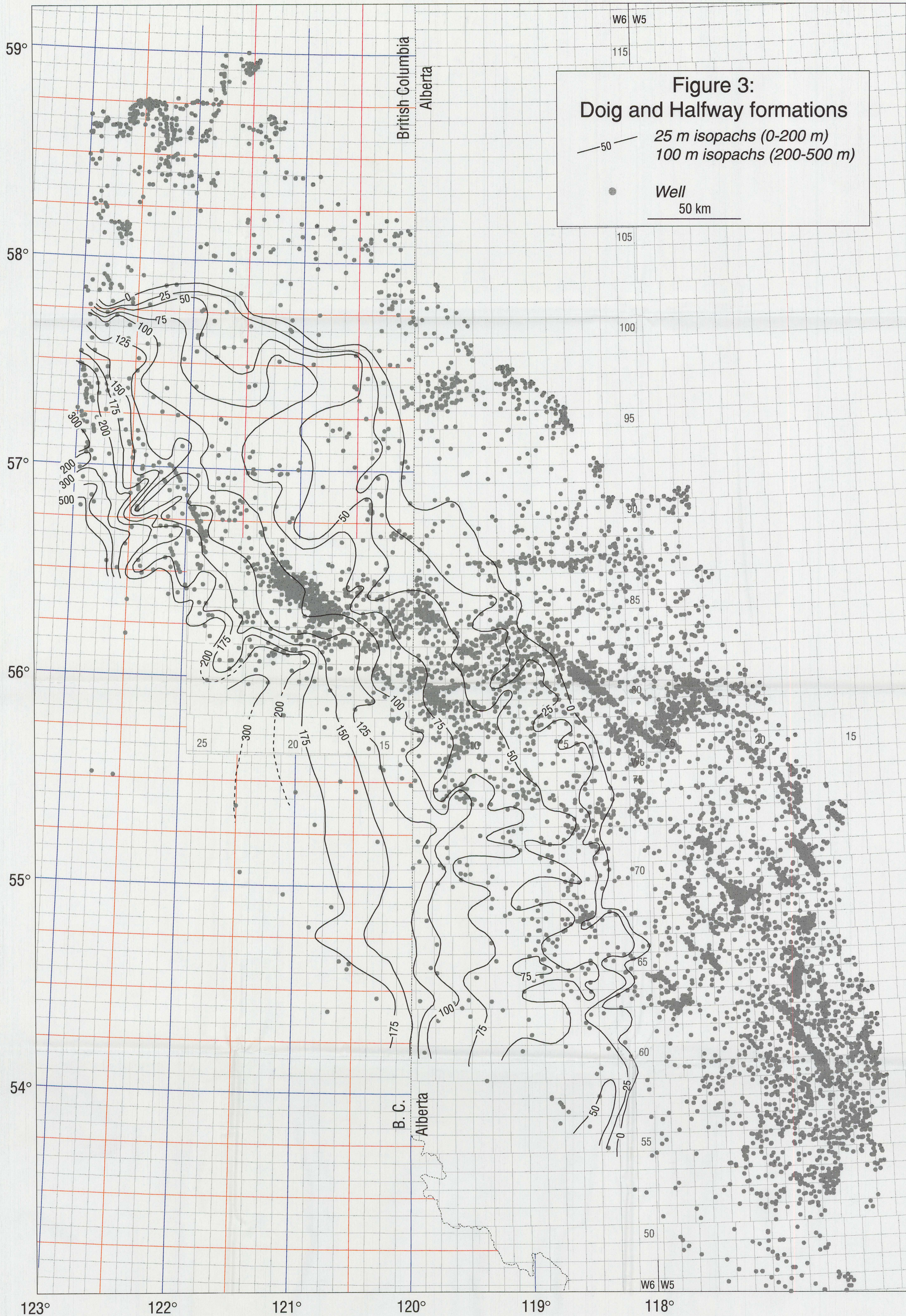
Isopach map of Doig and Halfway formations
