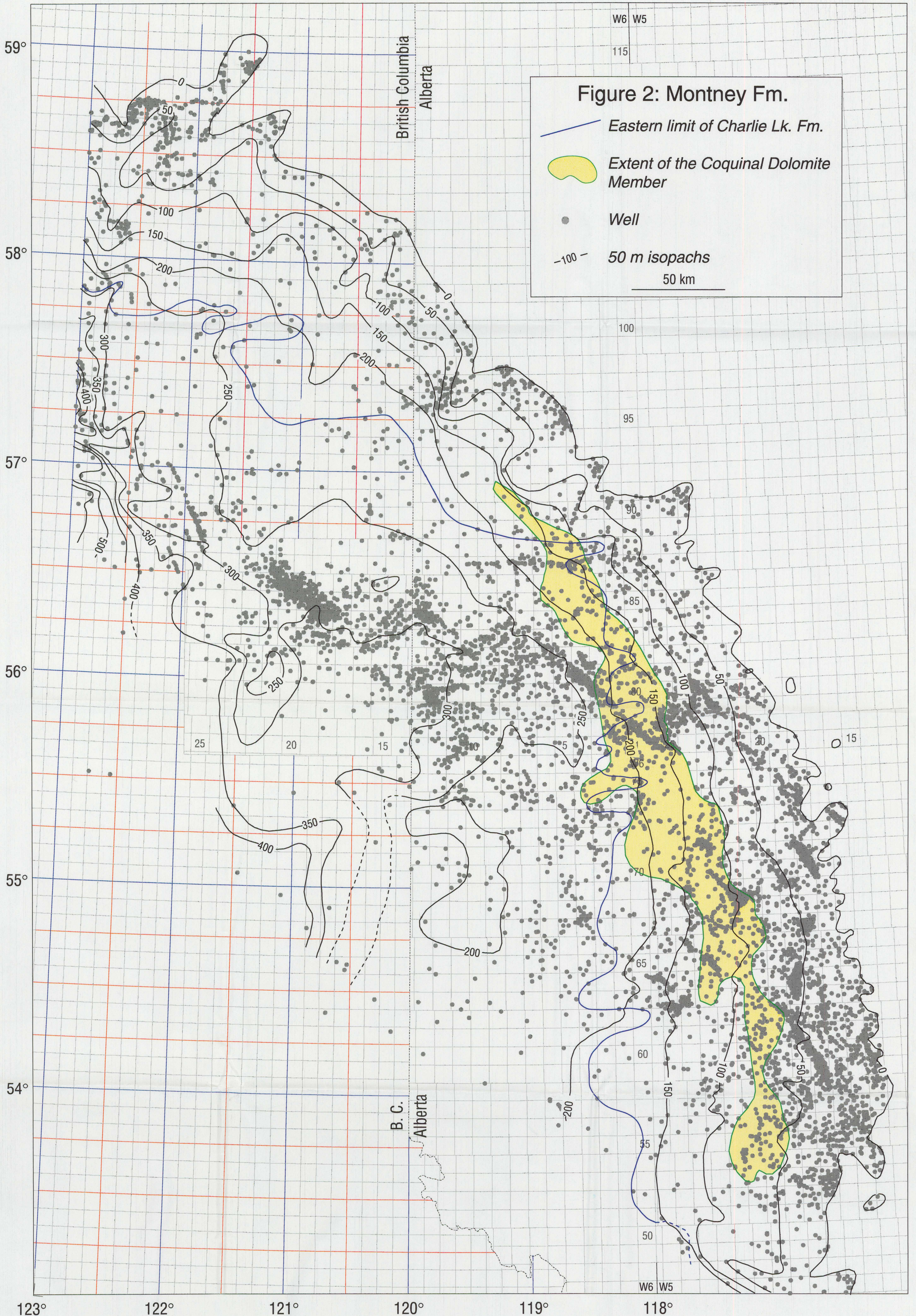
Isopach map of the Montney Formation
