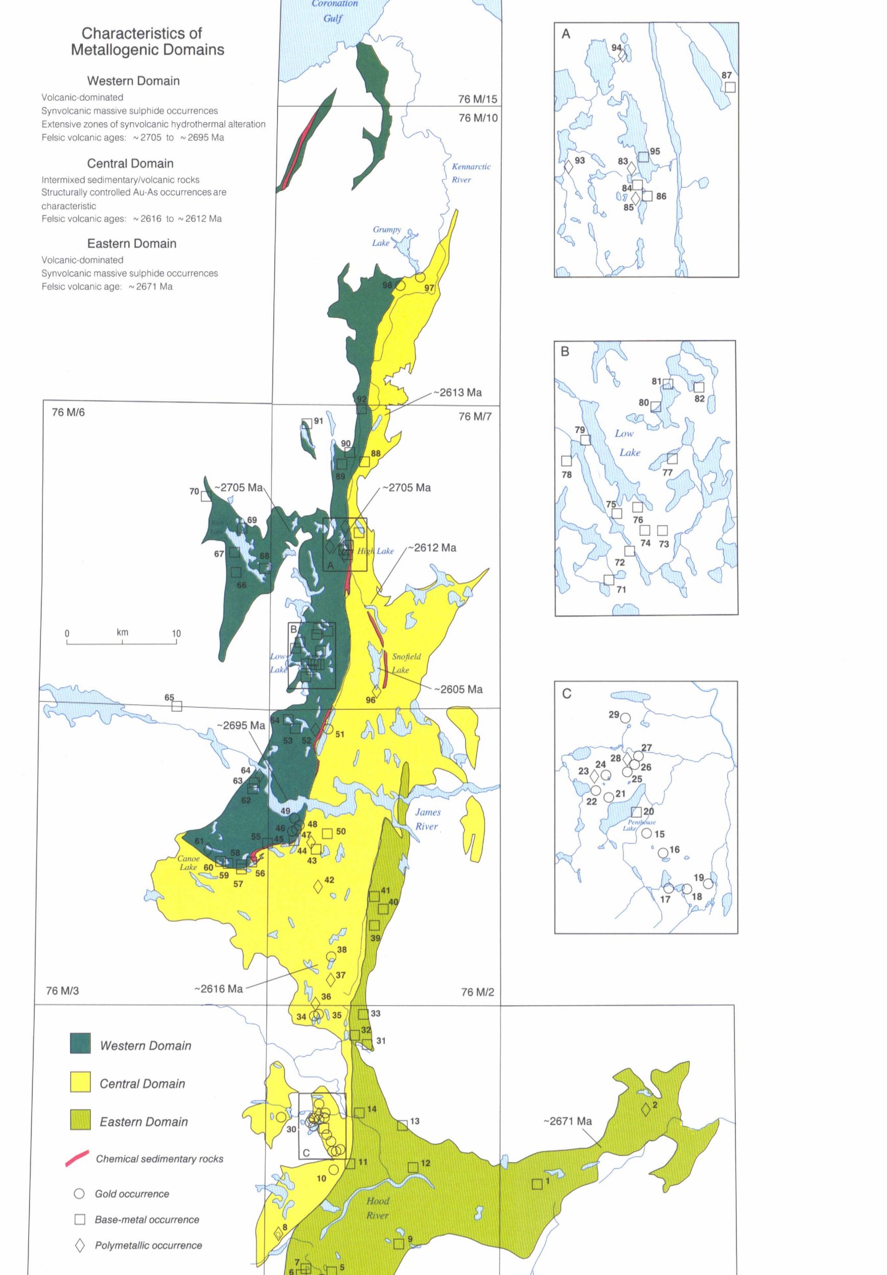
Figure 1. Metallogenic domain map
