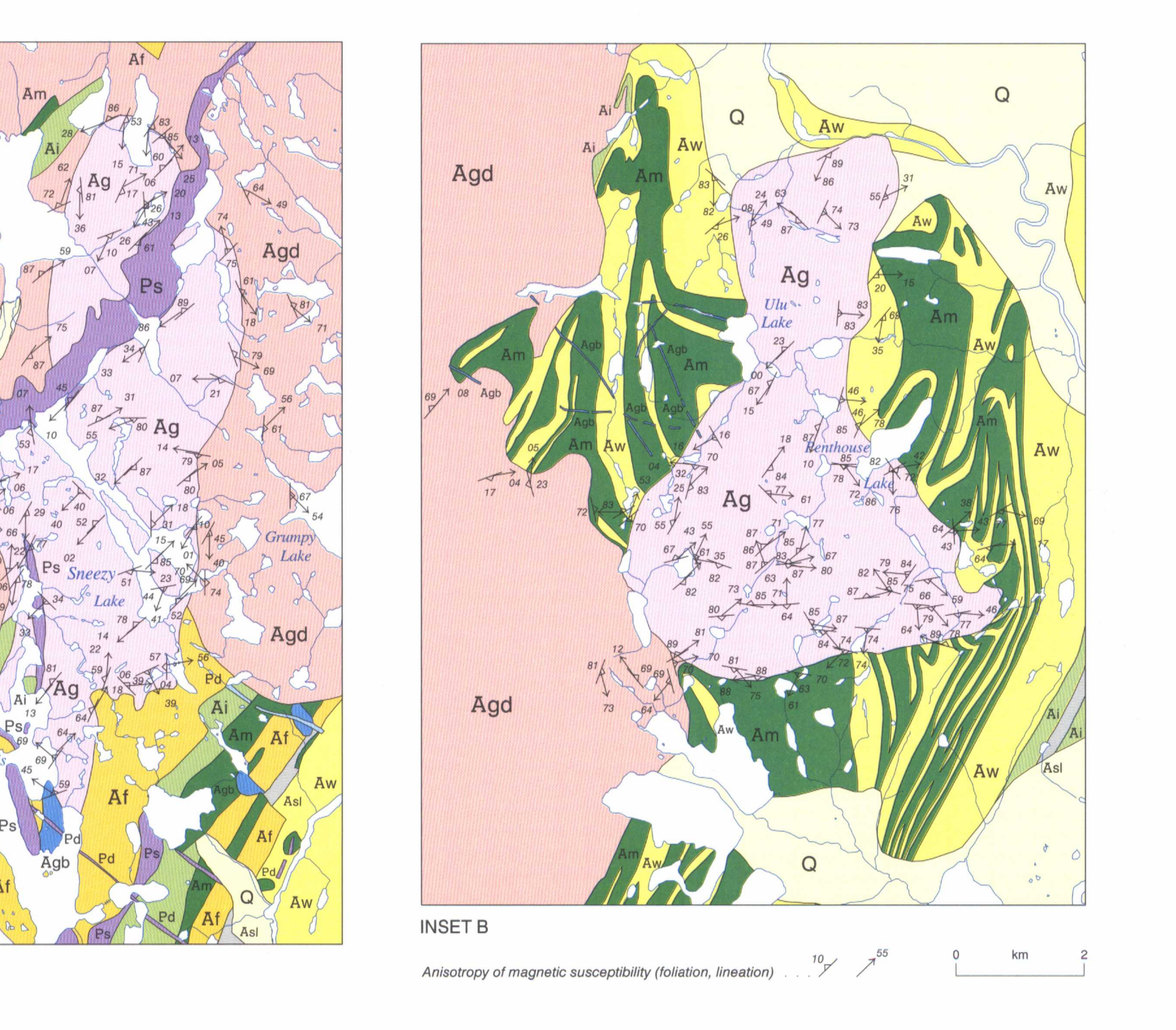
Inset A and Inset B showing detailed geological views.
