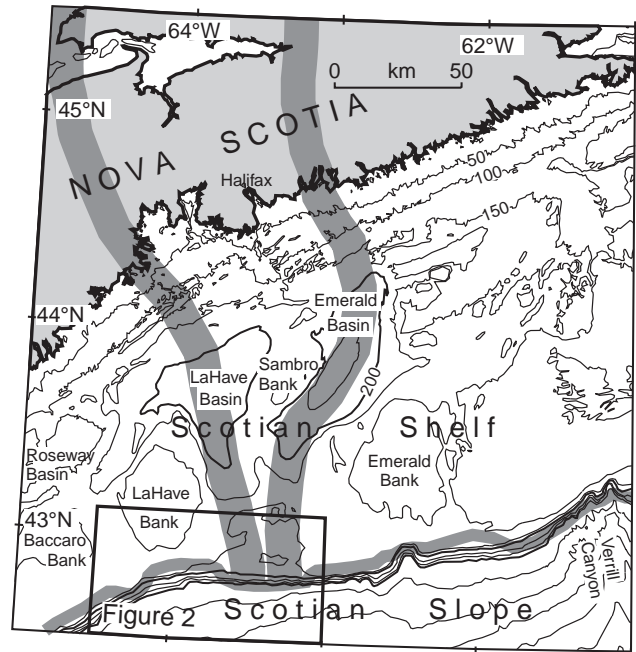
Figure 1. General map of Nova Scotia and the Scotian Shelf showing location of the study area (Fig. 2 box). Grey line at shelf edge represents late Wisconsinan ice margins (after Stea et al., 1998); thick grey bars represent position of ice streams (after Grant, 1989).
