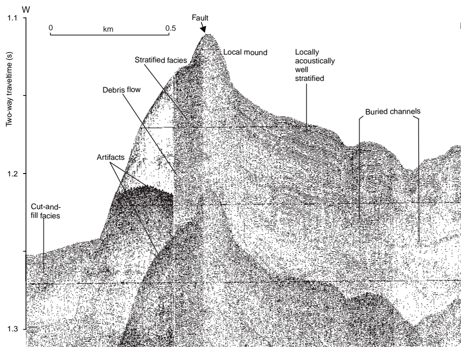
Figure 4. Hunttec DTS™ sparker high-resolution seismic profile of part of the section in Figure 3 showing greater seismic resolution of facies, cruise 99-036.
