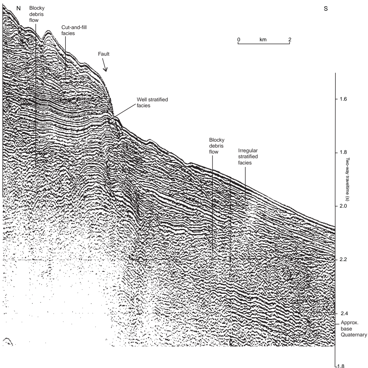
Figure 5. Seismic reflection profile down dip in zone A, showing facies, stratigraphy, and faulting. Two 40 cubic inch sleevegun source, cruise 99-036.
