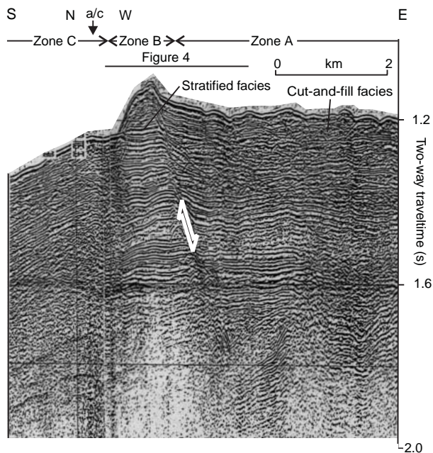
Figure 3. Seismic reflection profile along strike in 900 m water depth in zones A–C, showing facies, stratigraphy, and faulting. Two 40 cubic inch sleevegun source, cruise 99-036.
