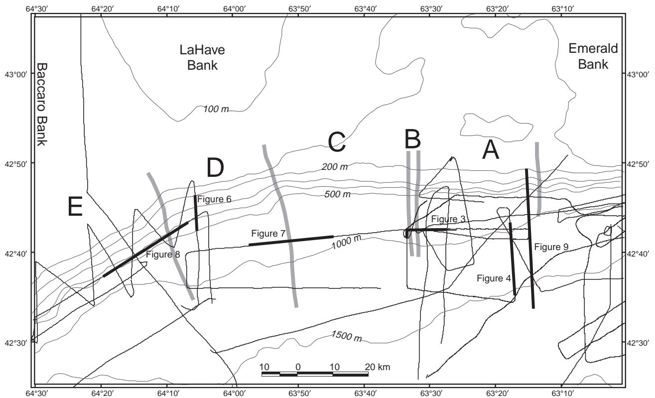
Figure 2. Map of study area showing seismic track lines and location of illustrated figures. 'A' to 'E' are zones discussed in text.
