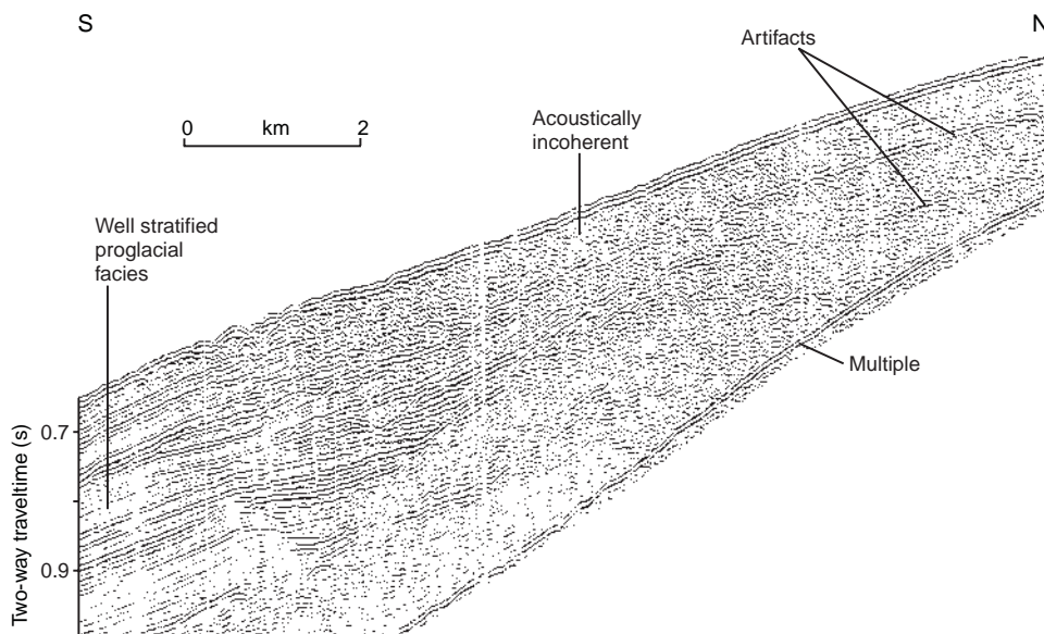
Figure 6. Seismic reflection profile down dip in zone D, showing incoherent acoustic facies corresponding to till passing downslope into well stratified acoustic facies, corresponding to proglacial plume fall-out deposits. One 40 cubic inch airgun source, cruise 90-002.
