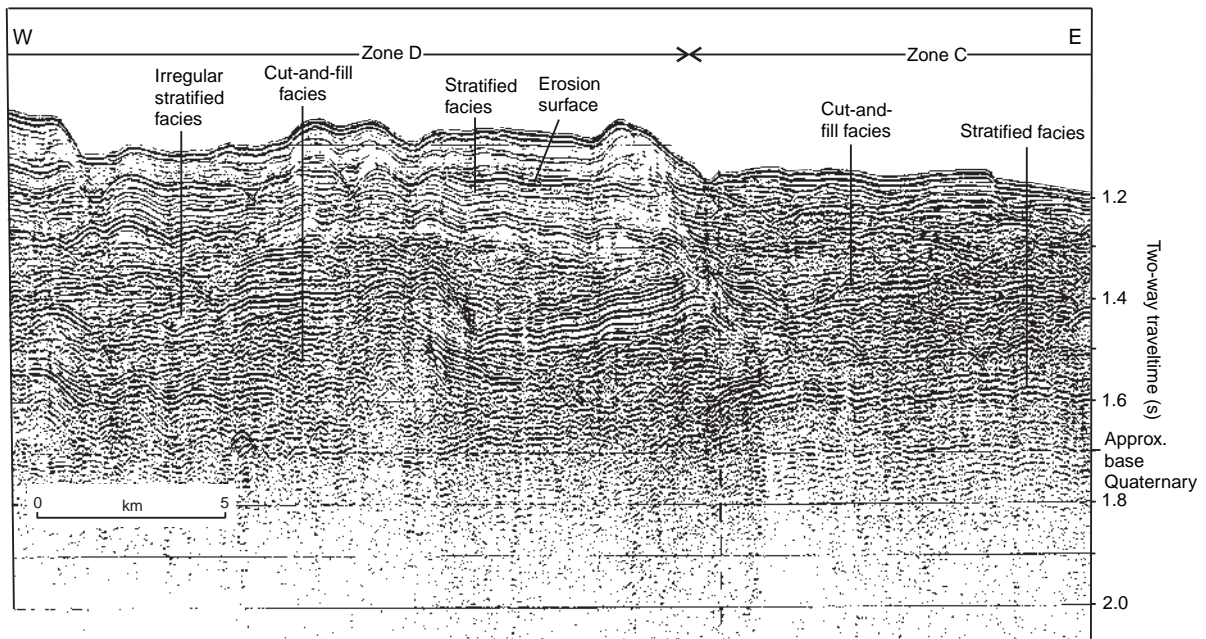
Figure 7. Seismic reflection profile along strike in 900 m water depth in zones C and D showing facies and stratigraphy. One 40 cubic inch sleevegun source, cruise 90-015.
