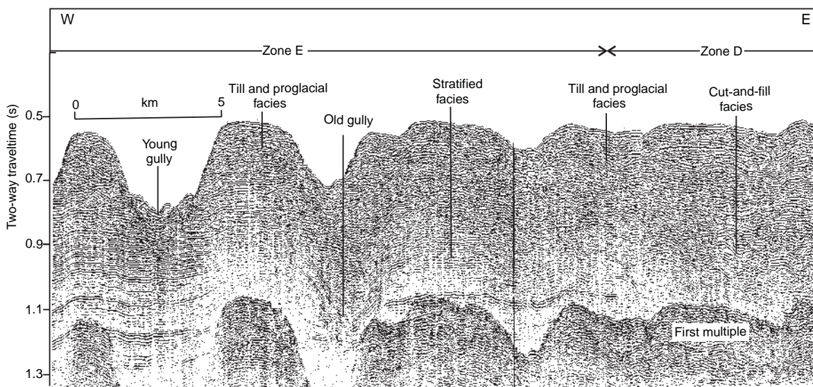
Figure 8. Seismic reflection profile along strike in 400 m water depth in zones D and E, showing gullies cutting till and proglacial facies overlying well stratified facies in zone E whereas in zone D, till and proglacial facies lack gullies and overlie cut-and-fill facies. One 40 cubic inch airgun source, cruise 90-002.
