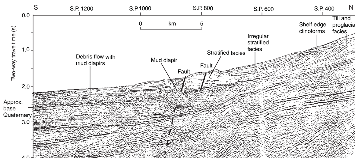
Figure 9. Industry multichannel seismic reflection profile down dip from the eastern end of zone A, showing late Cenozoic stratigraphy and facies. Petrocanada line 3416-82P courtesy Canada–Nova Scotia Offshore Petroleum Board.
