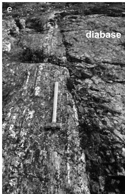
Figure 3. e) Late-synkinematic diabase obliquely cutting mylonite, and is itself mylonitized. f) Mafic granulite ultramylonite. g) Sinistral delta-winged felspar porphyroclast in amphibolite mylonite in Big lake shear zone west of Squiggly lake. h) Dextral shear-drag fold of quartz vein in the Ippijuaq Bay fault zone.
