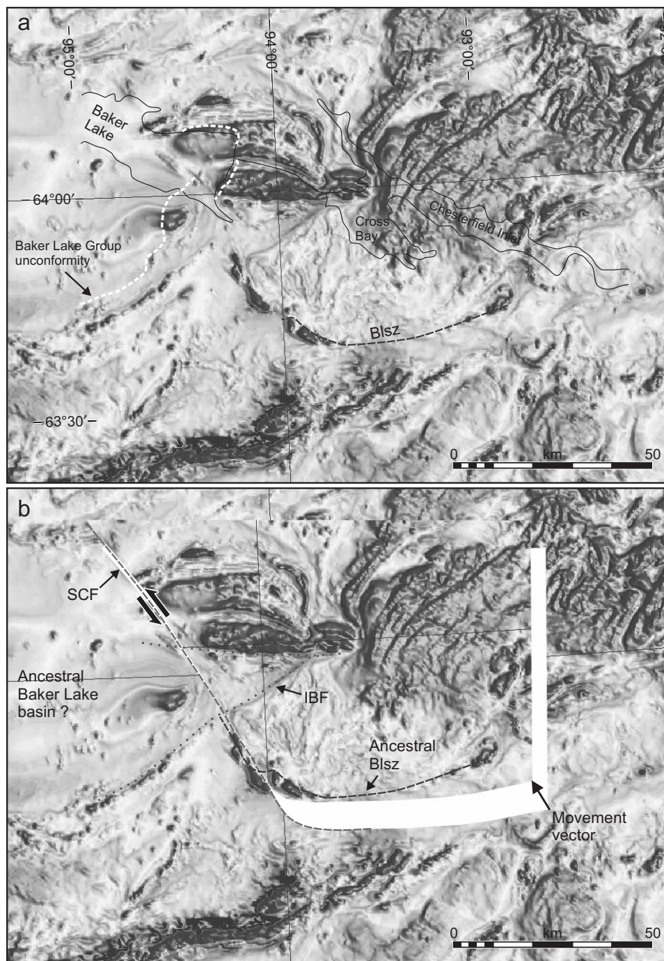
Figure 5. Shaded total field aeromagnetic map of the study area, encompassing Gibson Lake–MacQuoid Lake–Baker Lake–Chesterfield Inlet area (illumination from the east). a) Original aeromagnetic map. b) Restored aeromagnetic map, resulting from displacing the northwest block by 10 km to the northwest. Blsz=Big lake shear zone, IBF= Ippijuaq Bay fault, SCF=South Channel fault.
