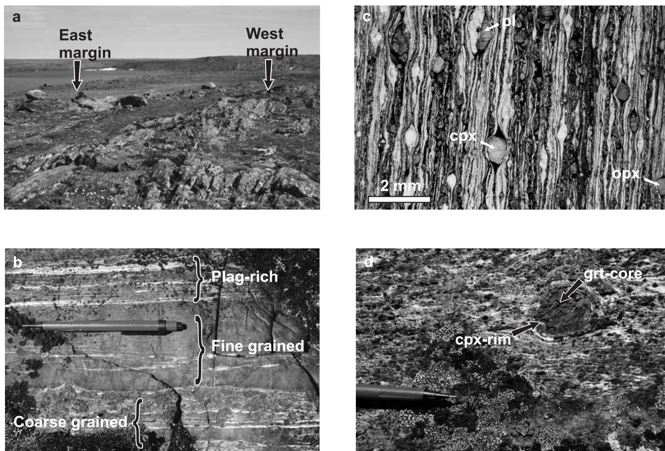
Figure 3. a ) Ten metre thick layer of anorthositic mylonite (light coloured) in the Big lake shear zone. b ) Compositionally layered mafic granulite gneiss, of variable grain size, in the Big lake shear zone; Plag=plagioclase. c ) Photomicrograph of mafic granulite ribbon ultramylonite. Garnet porphyroclasts are smaller than clinopyroxene (cpx), orthopyroxene (opx), and plagioclase (pl). d ) Composite garnet-clinopyroxene porphyroclast in coarse-grained granulite mylonite.
