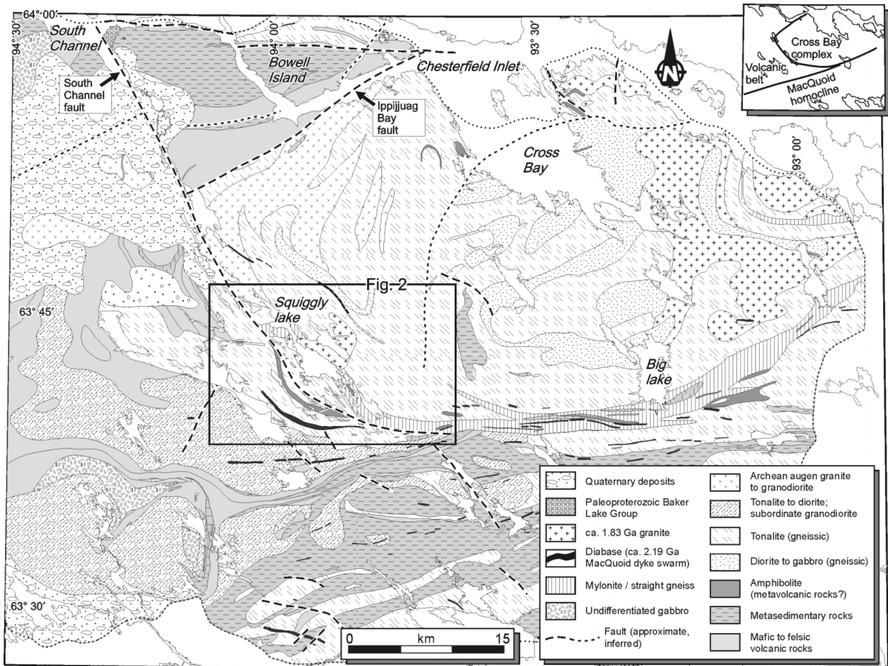
Figure 1. Generalized map of the Gibson Lake–Cross Bay–MacQuoid Lake area (after Tella et al., 1999). The location of Figure 2 is outlined. Note the location of the South Channel fault and the Ippijuaq Bay fault.
