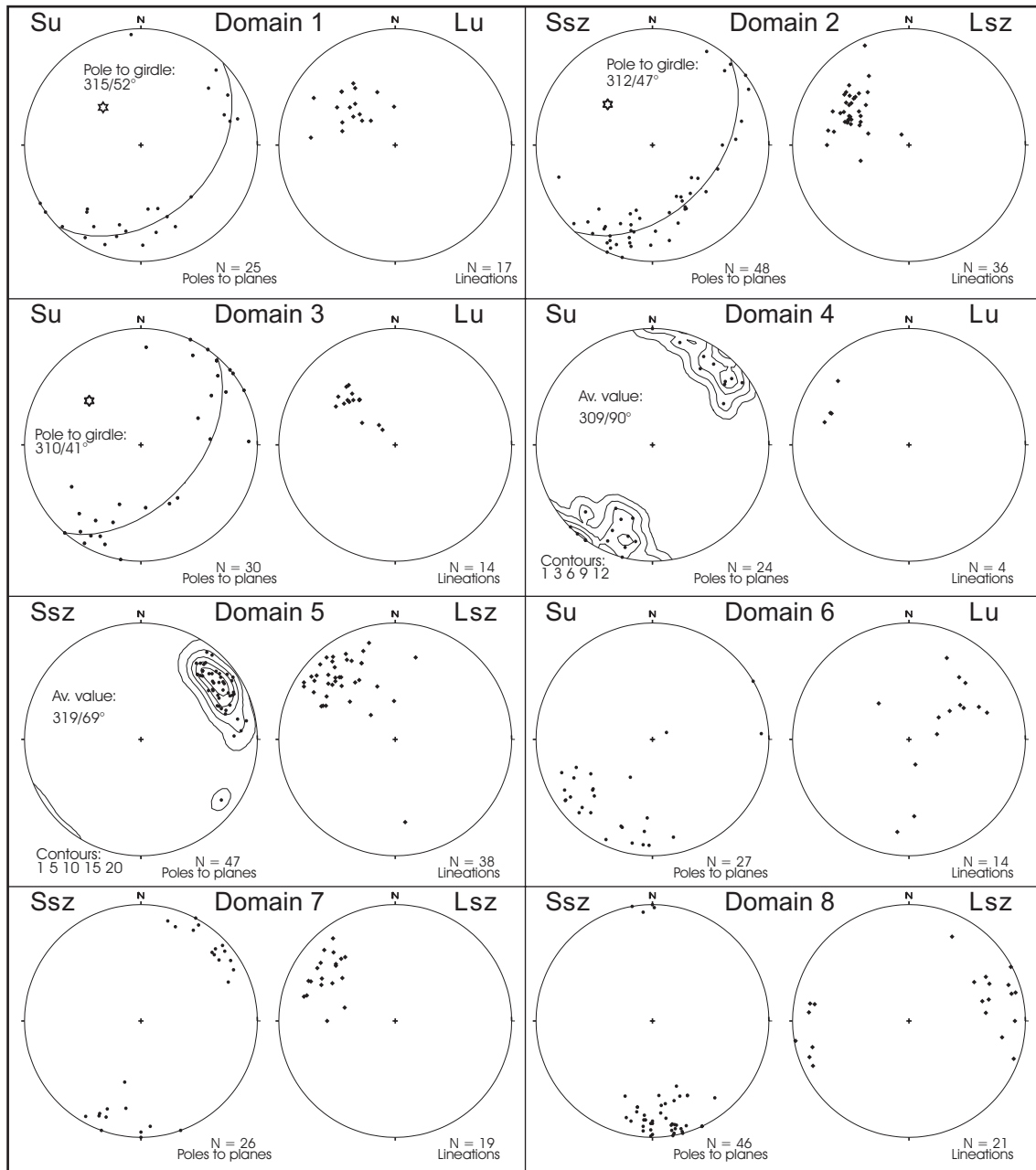
Figure 4. Lower hemisphere equal area projections of planar and linear fabric elements from the eight structural domains outlined in the Squiggly lake area ( see Fig. 2).
