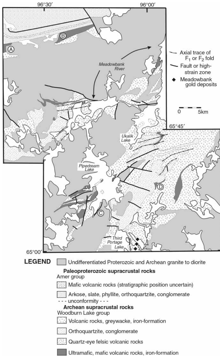
Figure 2. Generalized geology of the Woodburn Lake group from Third Portage Lake to the Amer belt. The geology of the Amer group is based partly on Patterson (1986). The circled letters refer to localities discussed in the text.
