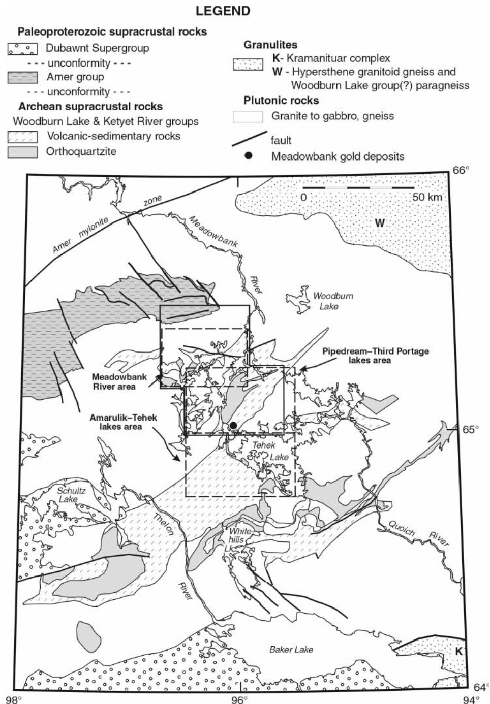
Figure 1. Regional setting of the Woodburn Lake and Ketyet River groups in the Amer Lake (NTS 66 H), Woodburn Lake (NTS 56 E), Baker Lake (NTS 56 D) and Schultz Lake (NTS 66 A) areas. The Ketyet River group includes quartzite and associated rocks from the Thelon River to the Quoich River. Dashed rectangles outline maps produced by the Woodburn Project, including the Meadowbank River area (Zaleski et al., 1999c, d), the Pipedream-Third Portage lakes area (Zaleski et al., 1997a, b) encompassing the Meadowbank gold deposits, and the Amarulik-Tehek lakes area (Zaleski et al., 1999a, b). The area of Fig. 2 is shown by a continuous line. The regional map is adapted from an unpublished compilation (L. Wilkinson, 1997) based on Donaldson (1966), Schau (1983), Fraser (1988), Taylor (1985), Tella (1994), and a compilation map in progress for the Schultz Lake area based on unpublished mapping by GSC geologists.
