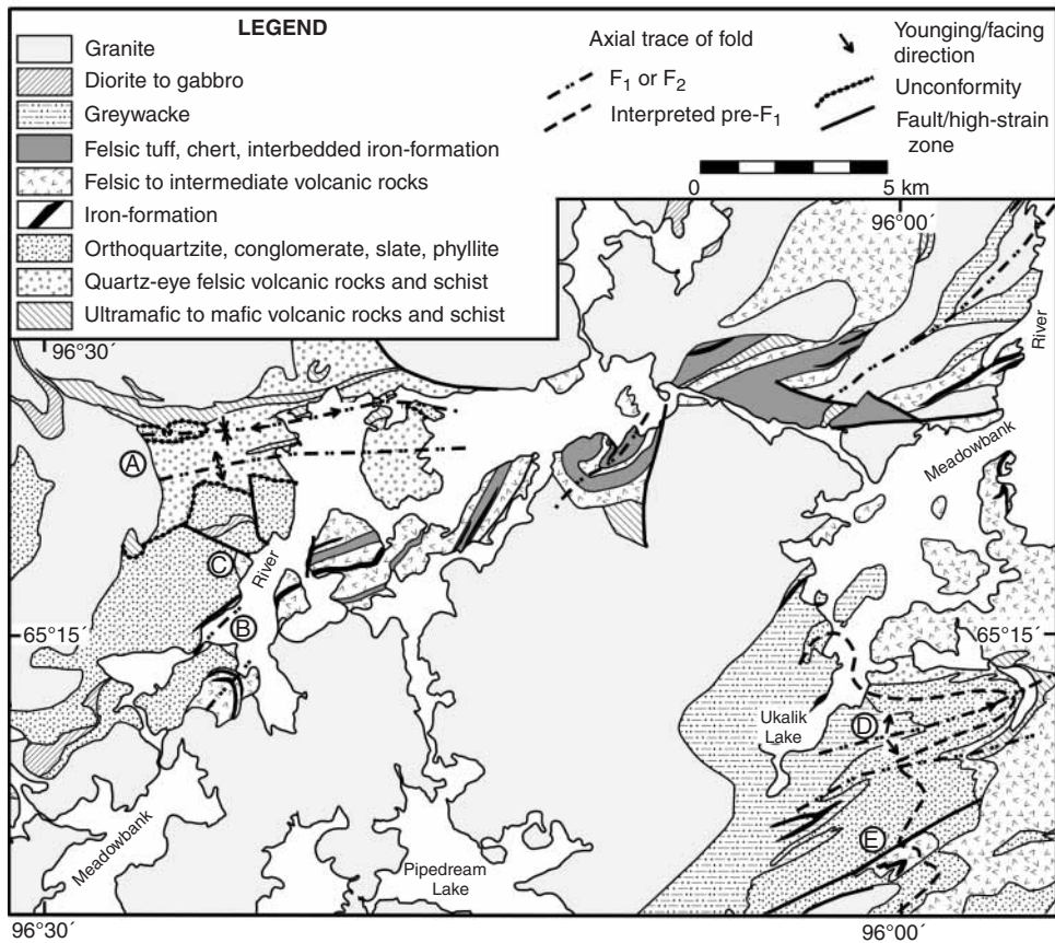
Figure 4. Generalized geology of the Woodburn Lake group from the Meadowbank River to Ukalik Lake. The circled letters refer to localities discussed in the text.
