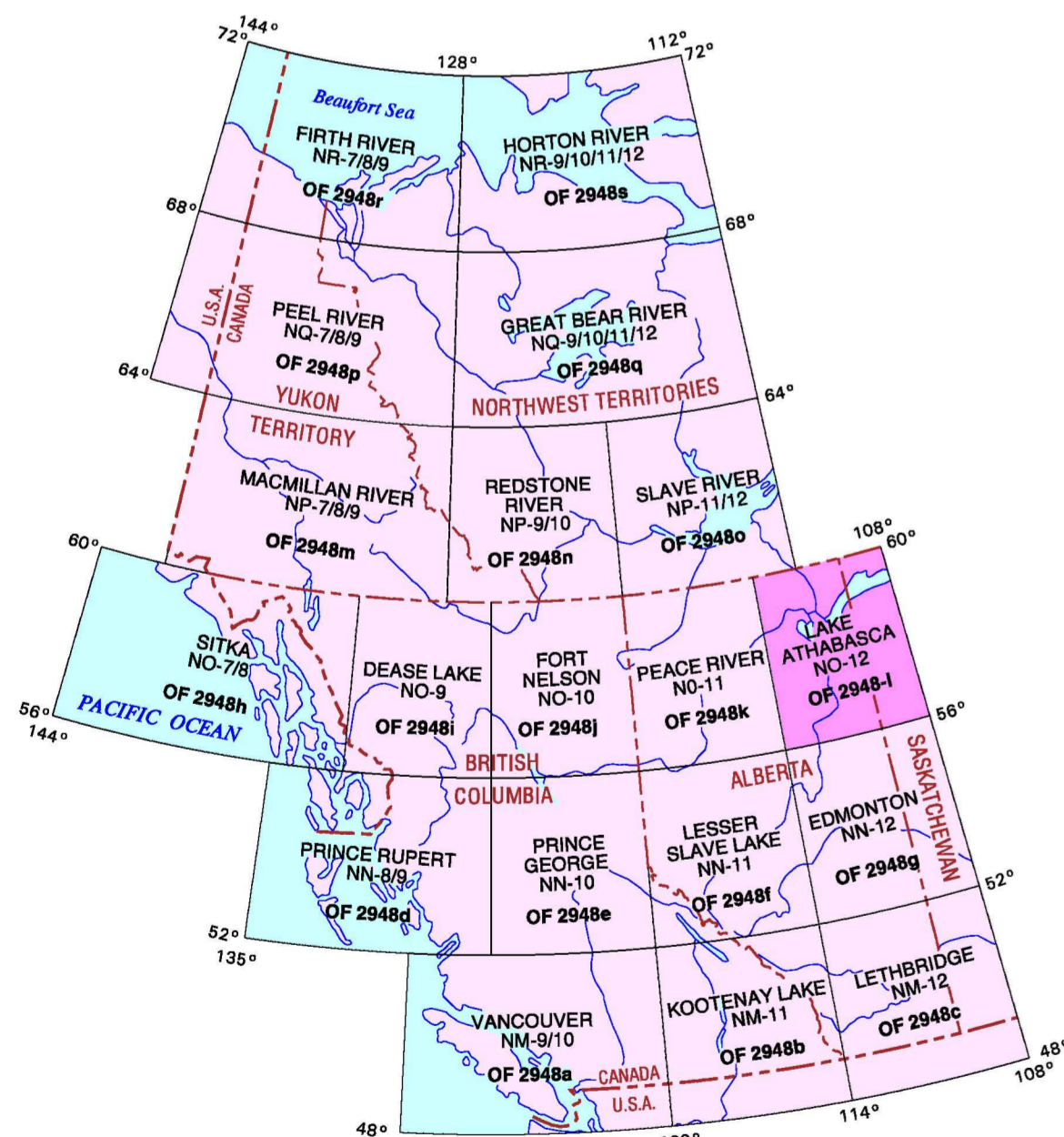
TECTONIC ASSEMBLAGES OF THE LAKE ATHABASCA MAP AREA 1:1 000 000 GSC OPEN FILE 2948-1
