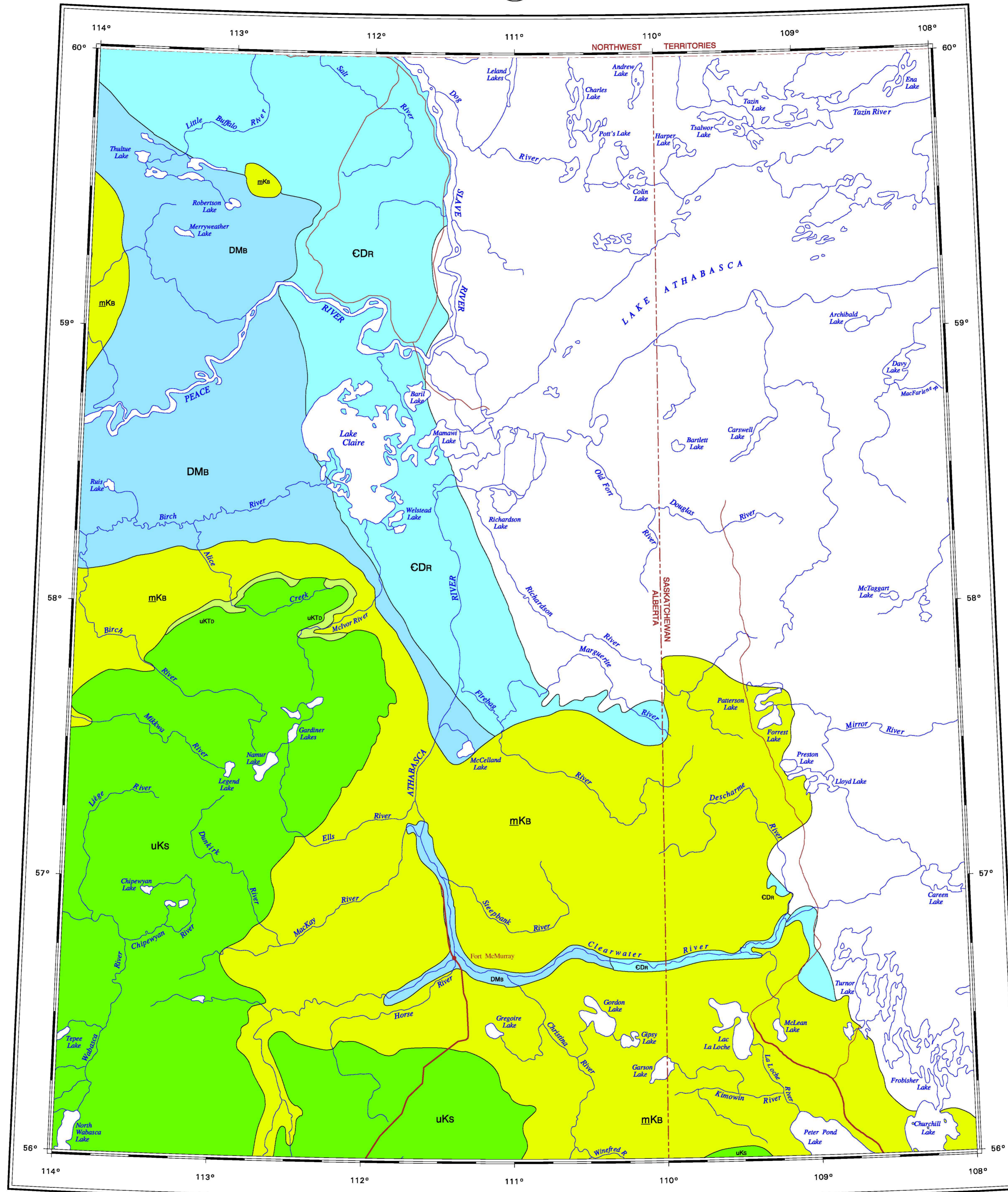
OPEN FILE 2948-1 TECTONIC ASSEMBLAGE MAP LAKE ATHABASCA ALBERTA - SASKATCHEWAN
