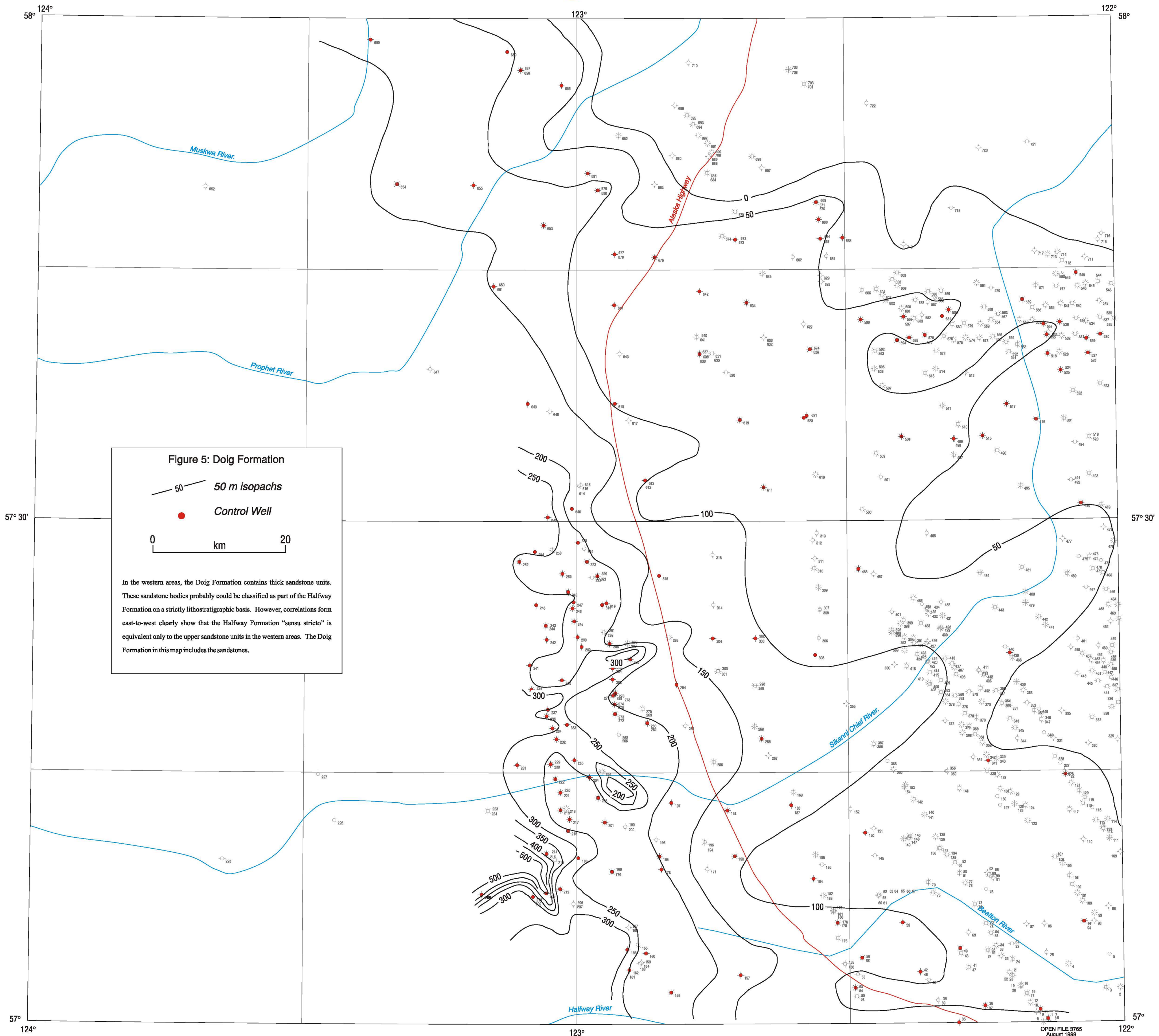
Isopach map of the Doig Formation
