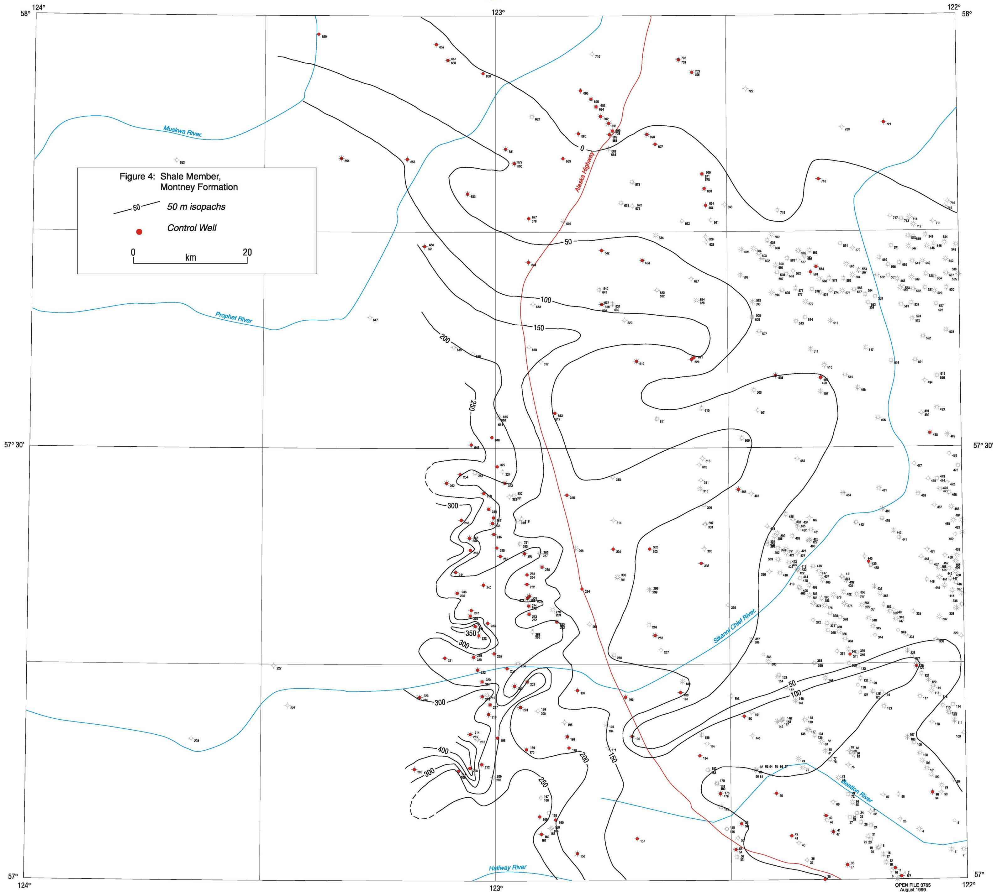
Isopach map of the Shale Member, Montney Formation
