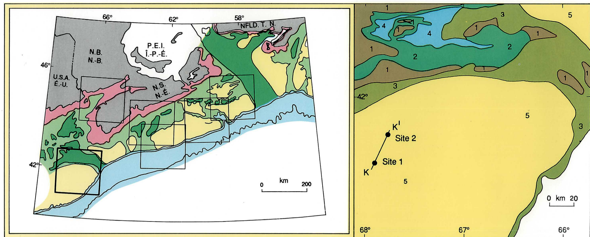
FIGURE 1. Index map, and surficial geology map (right, adapted from map sheet Surficial Geology and Physical Properties 5, this volume) showing location of cross-section K-K' and site locations, Georges Bank
