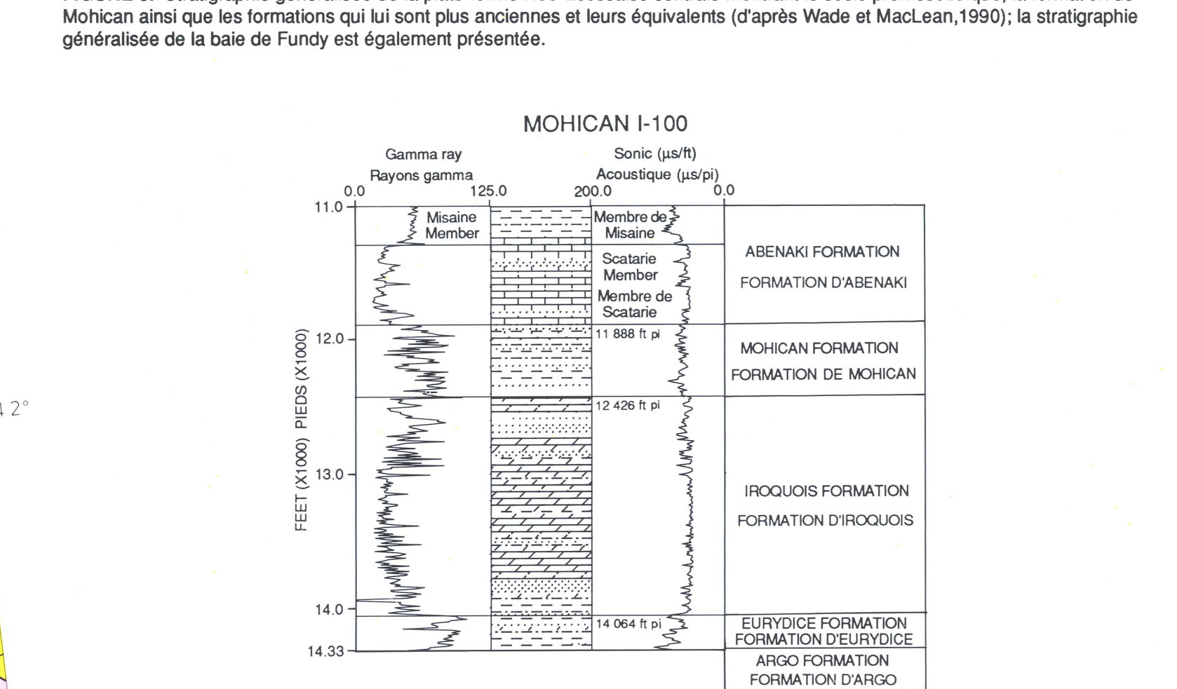
FIGURE 5. Type section, Iroquois and Mohican formations (location of well shown on Fig. 7) FIGURE 5. Stratotype, formations d'Iroquois et de Mohican (emplacement des puits indiqué à la fig. 7)
