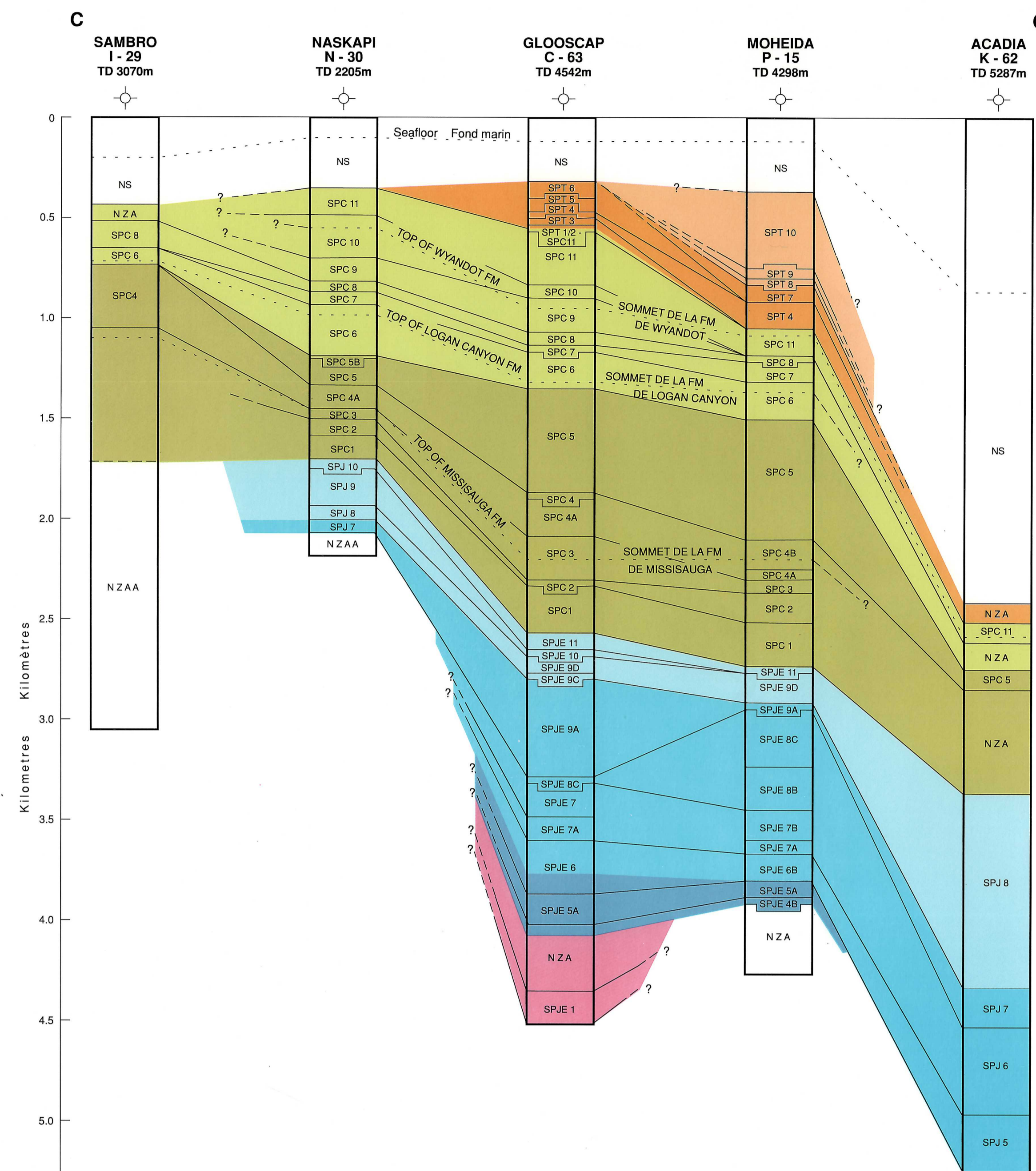
FIGURE 1. Palynostratigraphic cross-section C - C', Sambro I-29 to Acadia K-62 FIGURE 1. Coupe palynostratigraphique C - C', Sambro I-29 à Acadia K-62
