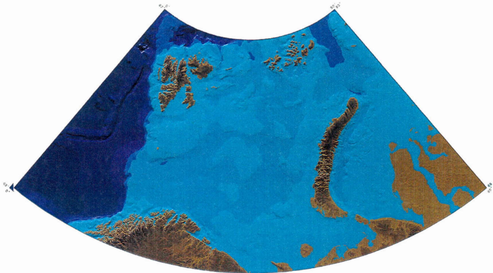
Bathymetric and Topographic Shaded Relief of the Barents and Kara Sea Region
