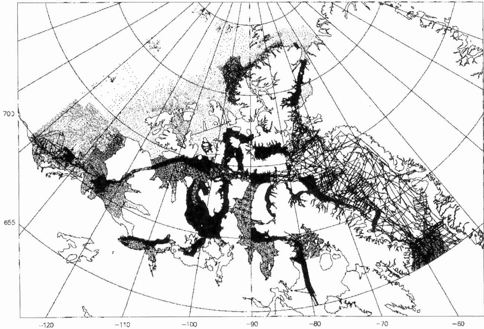
Figure 2. Locations of depth observations in and around the Canadian Arctic Archipelago, extracted from the digital archives of the Geological Survey of Canada and the Canadian Hydrographic Service. (Macnab)
